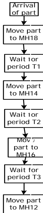
Figure 6: Flow chart for the auxiliary buffer
