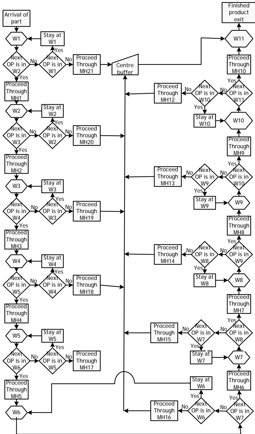
Figure 4: Flow chart for the designed reconfigurable manufacturing system - outside the auxiliary buffer
