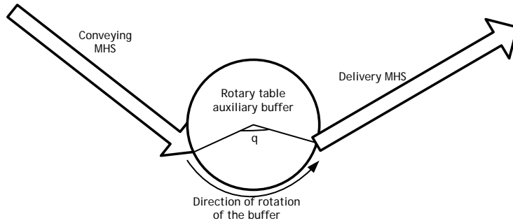
Figure 1: An iconic representation of suggested control method at the auxiliary buffer
