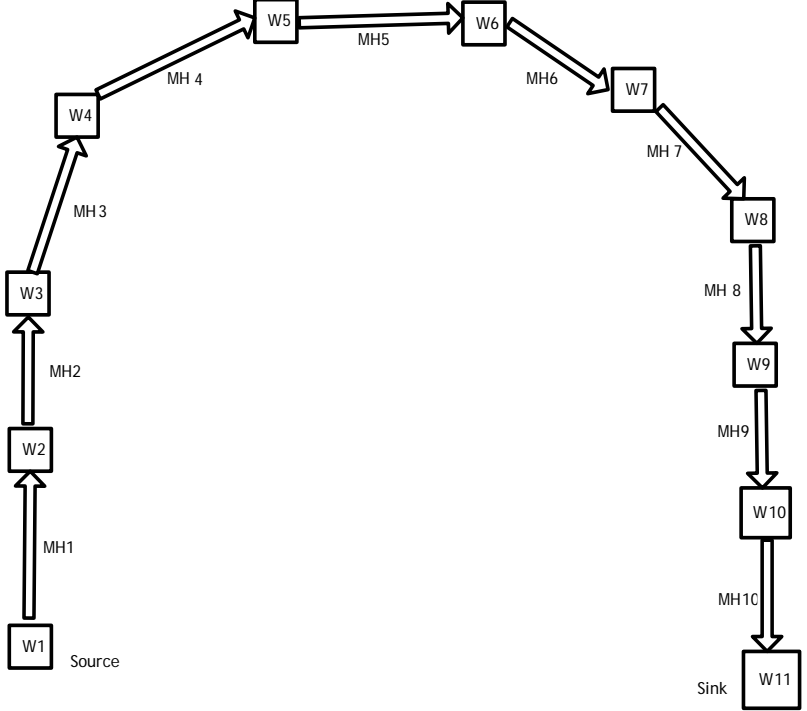
Figure 3: Original/Initial manufacturing system with provision for material-handling system (MH11-MH21) not displayed but available in the system for activation when necessary.
