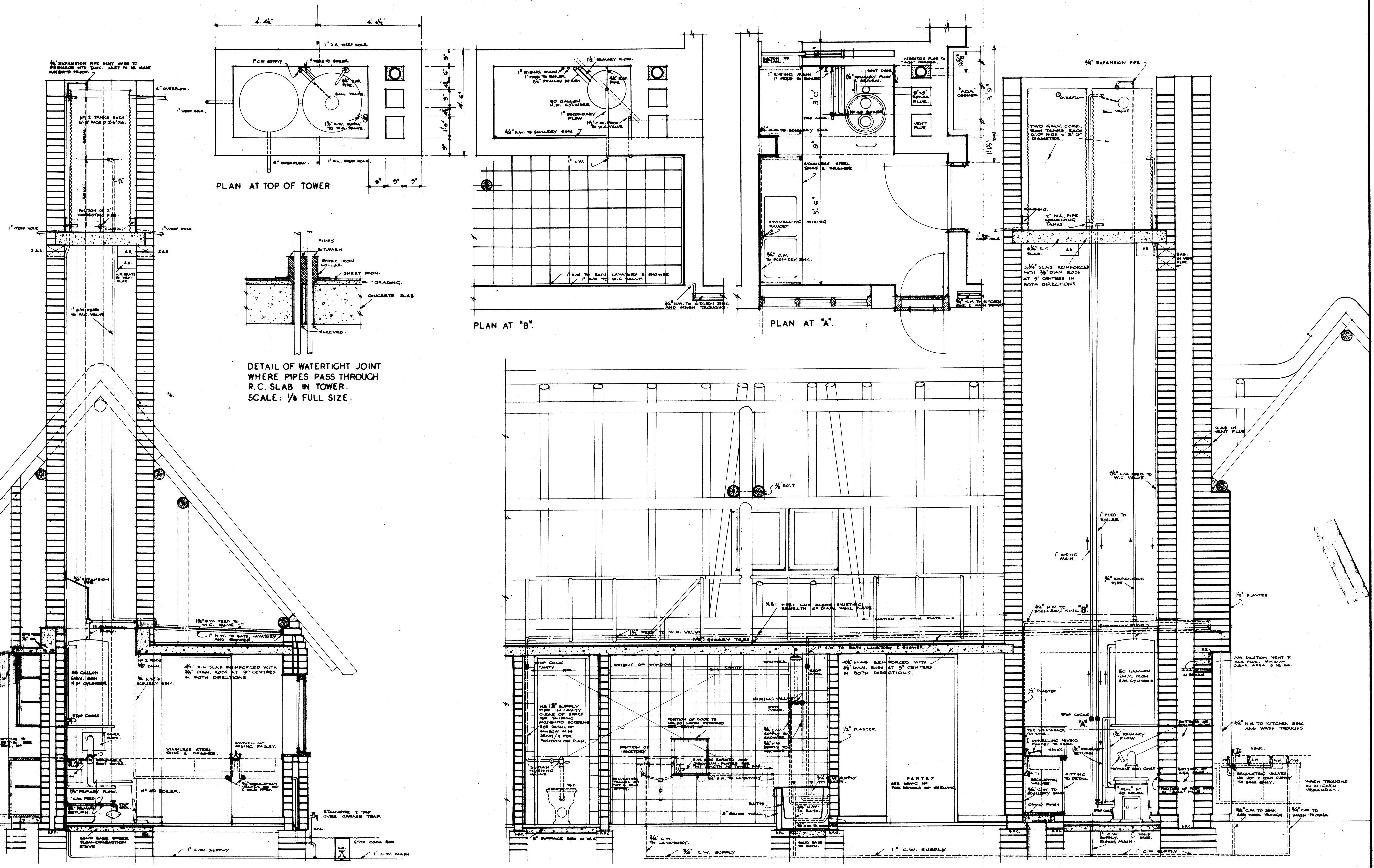
CROSS SECTION THROUGH TOWER, LOFT & SCULLERY.
