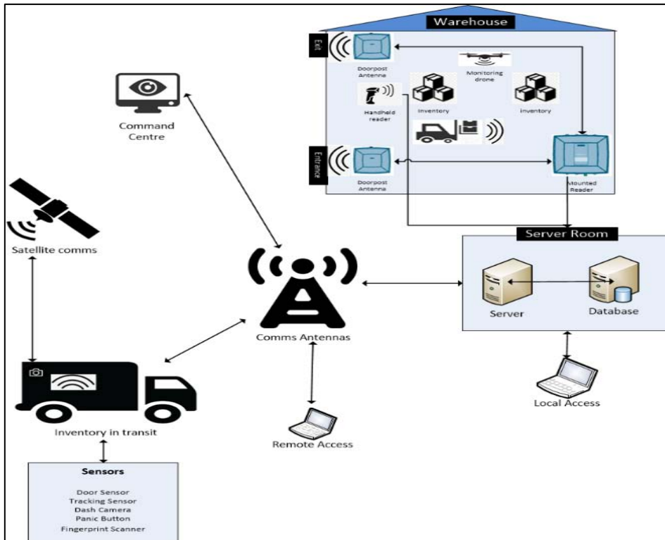
Figure 2: SWMS High Level Architecture
