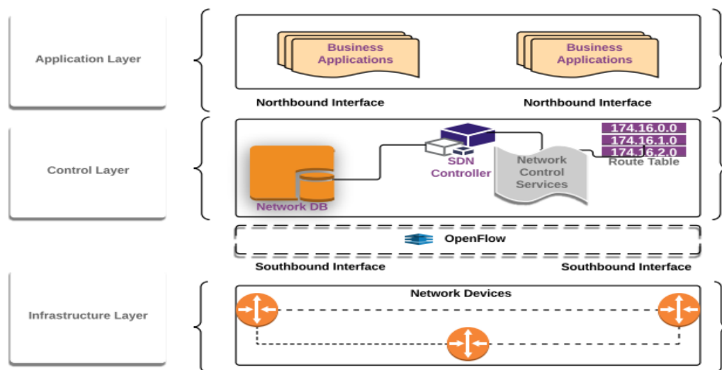
Figure 1. An overview of SDN architecture.
