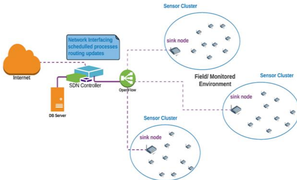
Figure 2: Software Defined Wireless Sensor Network Architecture.
