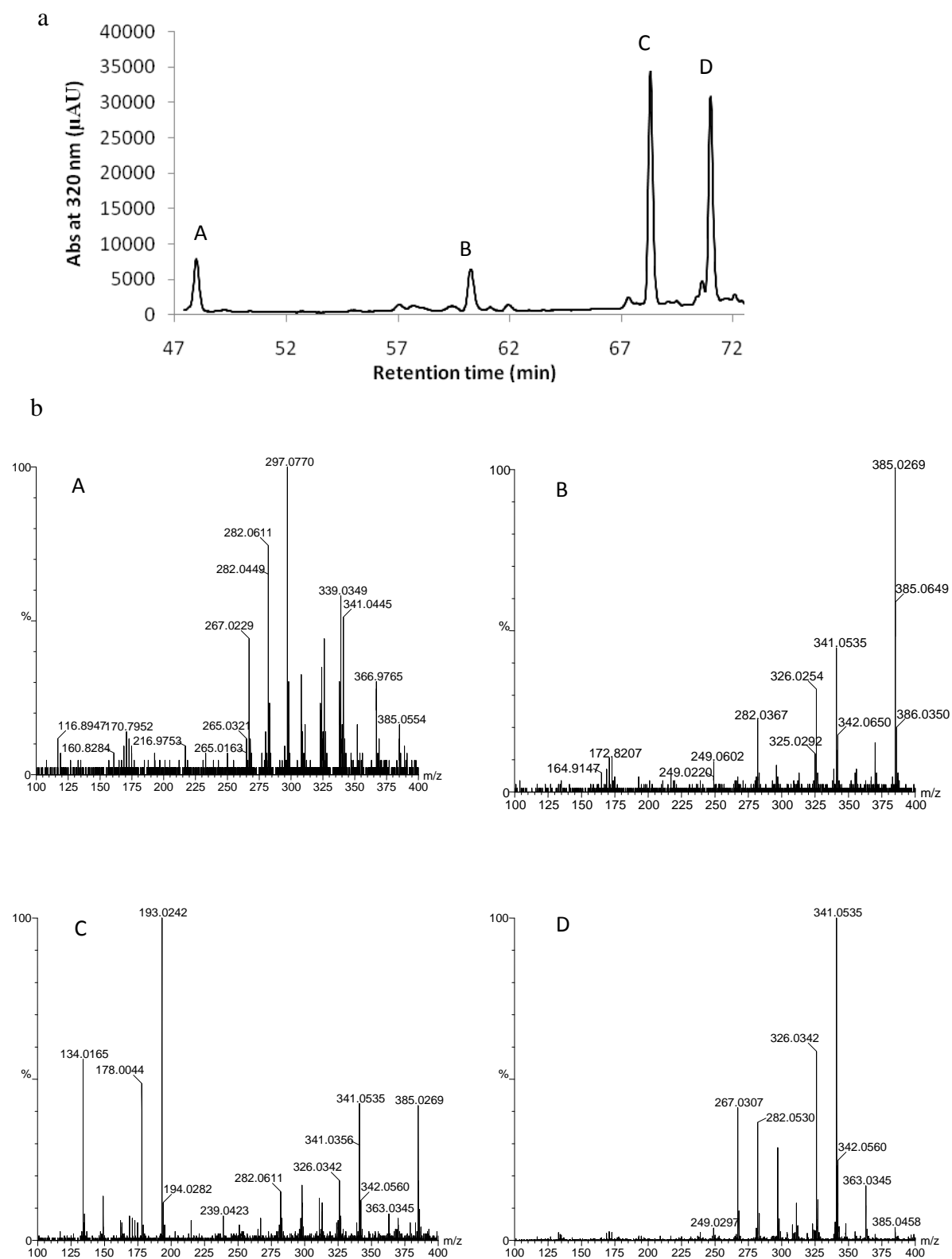
Figure 1. LC chromatogram (a) and MS/MS spectra (b) of diferulic acids 8-8' (A), 5-5' (B), 8-O-4' (C) and 8-5'benzofuran form (D), respectively from the sorghum cultivar PAN 8902.
