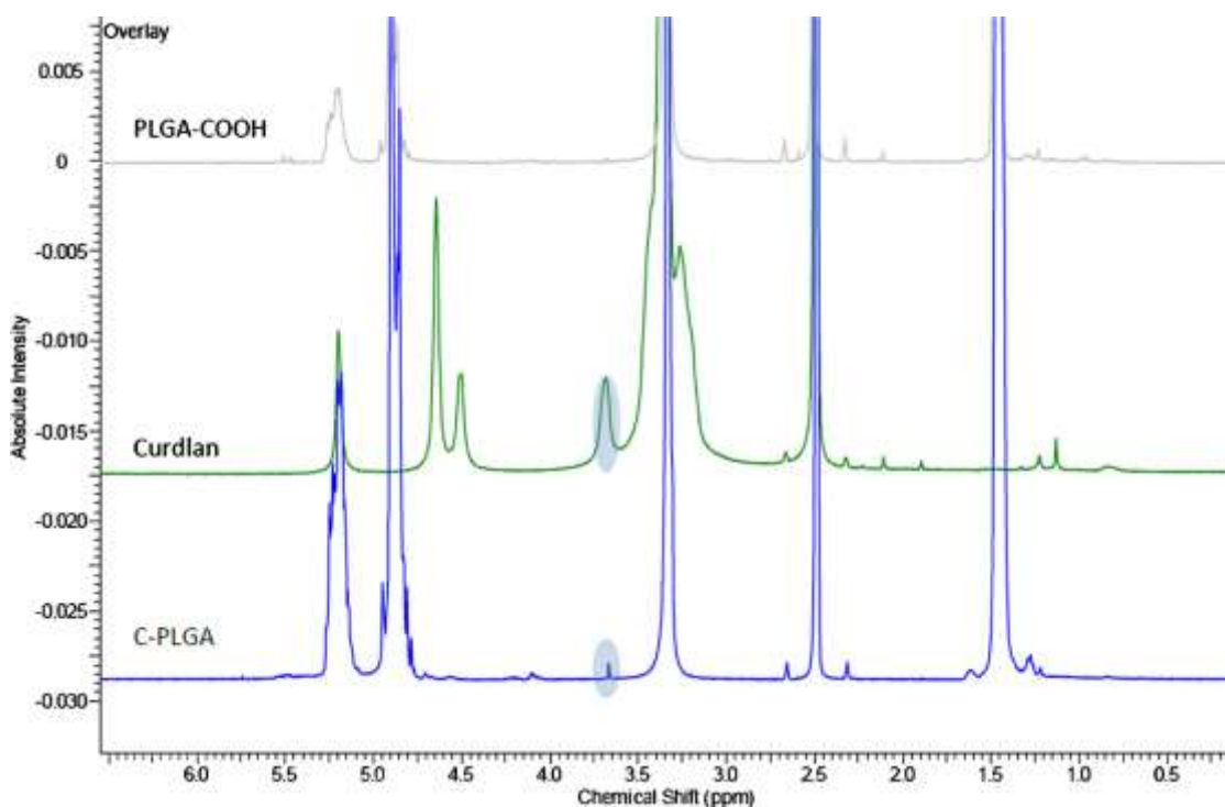
Figure 2: 1 H NMR spectra of PLGA-COOH, curdlan and C-PLGA copolymer. C-PLGA spectra reveals new peak (highlighted) at 3.69 ppm attributed to the presence of curdlan OCH 2 groups.
