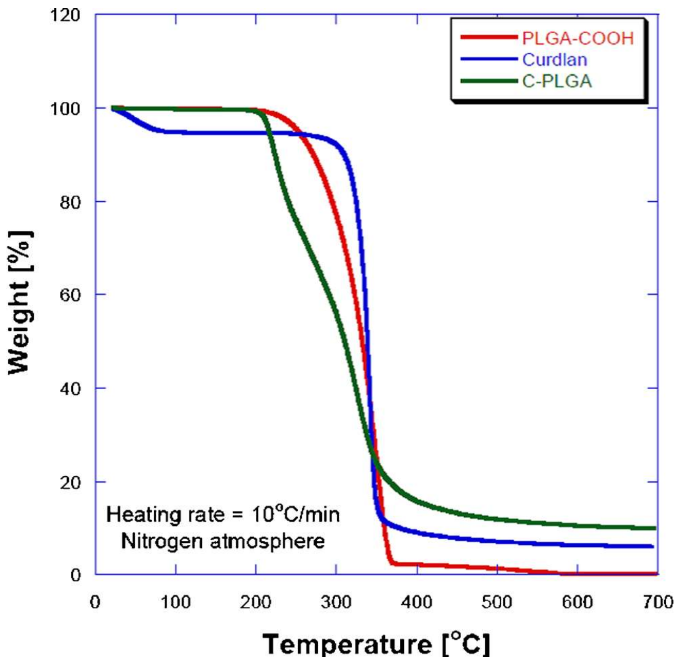
Figure 5: TGA thermogram curves of PLGA-COOH, curdlan and Curdlan-PLGA.
