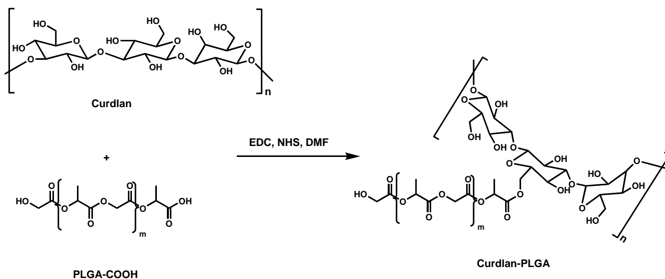
Figure 1: Schematic of synthesis of C-PLGA copolymer. Acid terminated PLGA is reacted with curdlan to produce C-PLGA conjugate ( Reagents and conditions: EDC.HCl, NHS, DIEA, DMF, rt, 48 h ).
