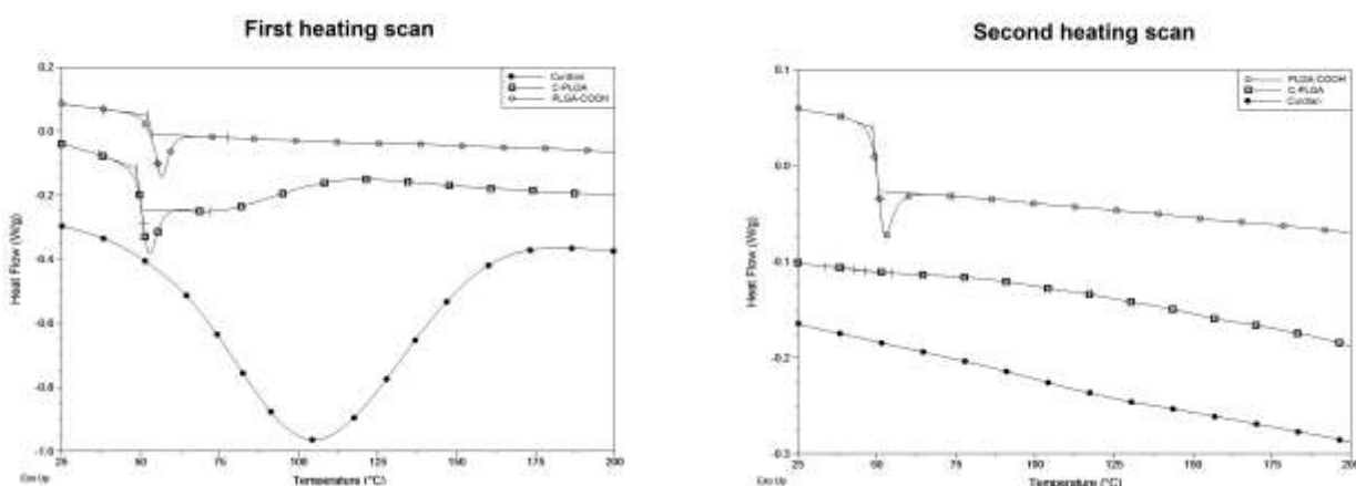
Figure 6: DSC curves (1st and 2nd melt) for PLGA-COOH, curdlan and Curdlan-PLGA.
