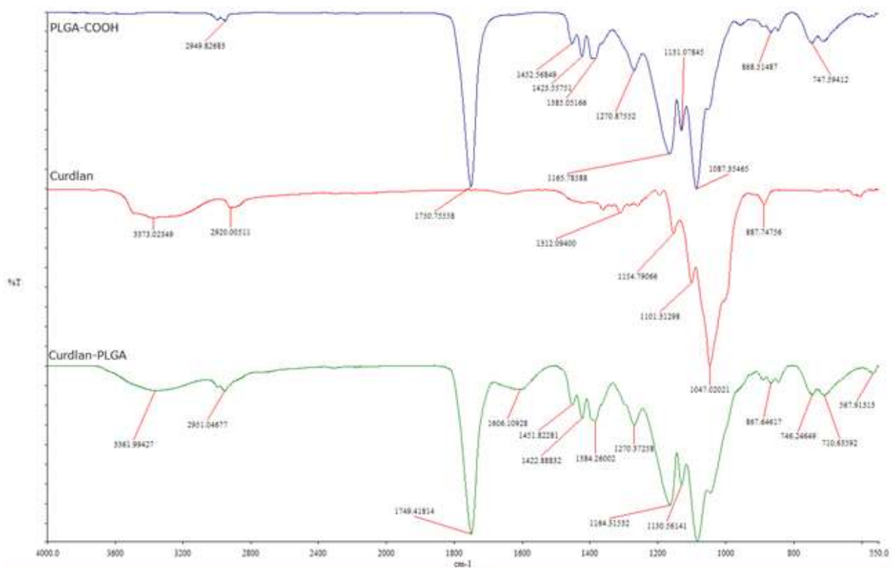
Figure 4: FT-IR spectra of acid terminated PLGA-COOH, curdlan and Curdlan-PLGA copolymer.
