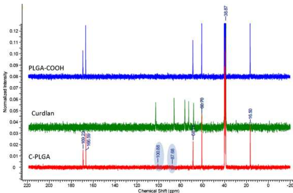
Figure 3: 13 C NMR spectra of PLGA-COOH, curdlan and C-PLGA copolymer. C-PLGA spectra reveals new peaks resonating at 87.7 and 100.9 ppm, attributed to the carbons of the curdlan backbone in the copolymer.
