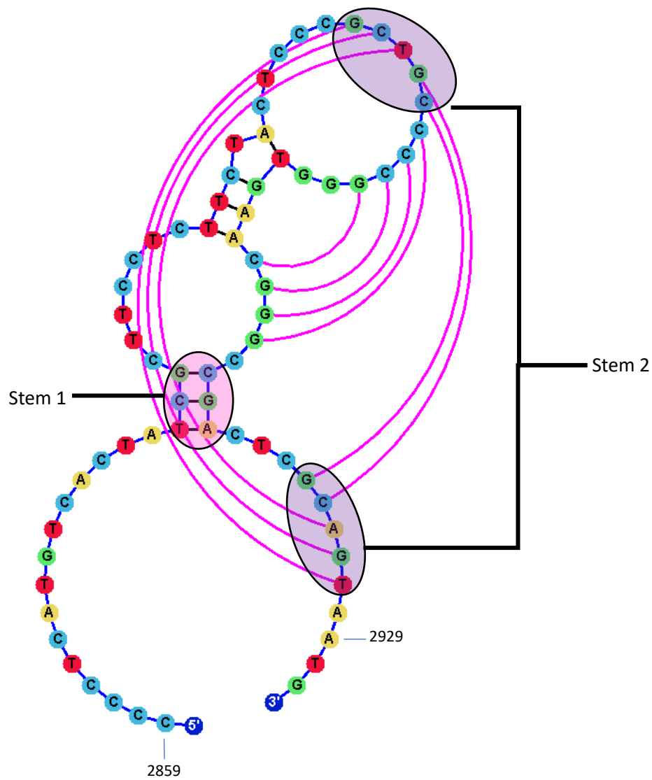
Fig S8. Predicted pseudoknot structure spanning the stop-start region of TpRV-2. The nucleotide positions are indicated. Stem 1 and Stem 2 are indicated by purple and pink ovals, respectively. Structures were predicted with ProbKnot and visualized with jViz.RNA 4.0.
