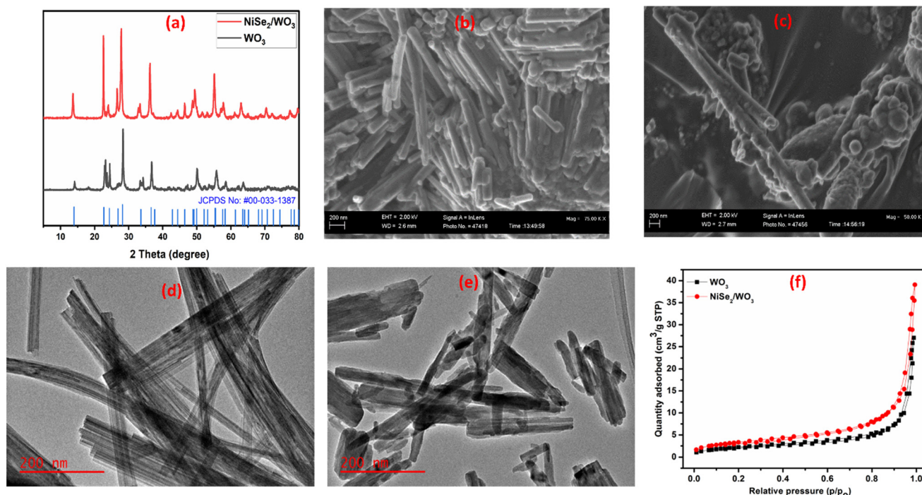
Fig. 1 a) XRD diffraction patterns of WO 3 and NiSe 2 /WO 3 , b) SEM image of WO 3 , c) SEM image of NiSe 2 /WO 3 , d) TEM image of WO 3 , e) TEM image of NiSe 2 /WO 3 , and f) N 2 sorption isotherms for WO 3 and NiSe 2 /WO 3 .
