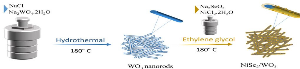
Scheme 1 Synthesis of the NiSe 2 /WO 3 heterojunction.
