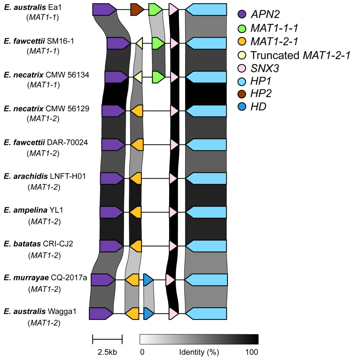
Figure S2. Diagram showing the structure of MAT1 locus of Elsinoe species using genome data – adapted from Pham et al. (2023).
