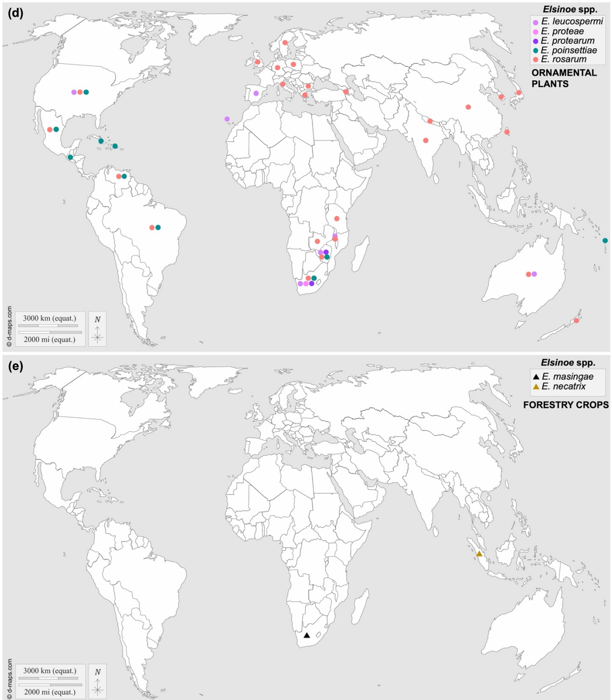
Figure S1. Worldwide distribution of Elsinoe spp. affecting economically important agricultural, ornamental and forestry crops. (a) Fruit crops; (b) Tuber crops; (c) Legumes crops; (d) Ornamental plants; and (e) Forest trees. Colours and symbols indicate the occurrence of Elsinoe spp. in each country. Data were captured from Table S1, EPPO Global database ( https://gd.eppo.int/ ), CABI Compendium ( https://www.cabidigitallibrary.org/ ), and USDA Fungus-Host Distributions database ( https://fungi.ars.usda.gov/ ).
