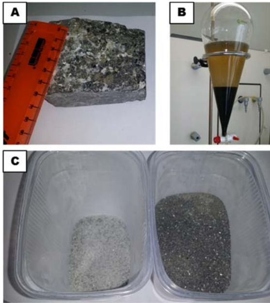
Fig. S1 Photographs of sample Plg-c in its pristine form (A), density separation setup (B), and density-separated fractions (C)
