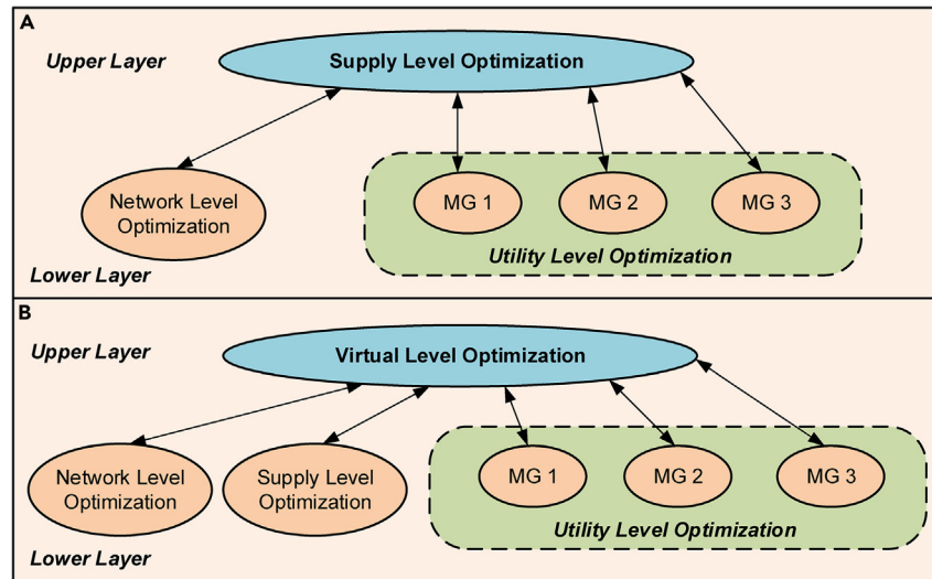
Figure 6. Conceptual scheduling optimization framework (A) sequential optimization (B) parallelizing optimization.
