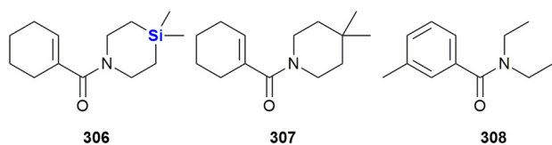
Fig. 92 Sila-piperidine amide mosquito repellent.
