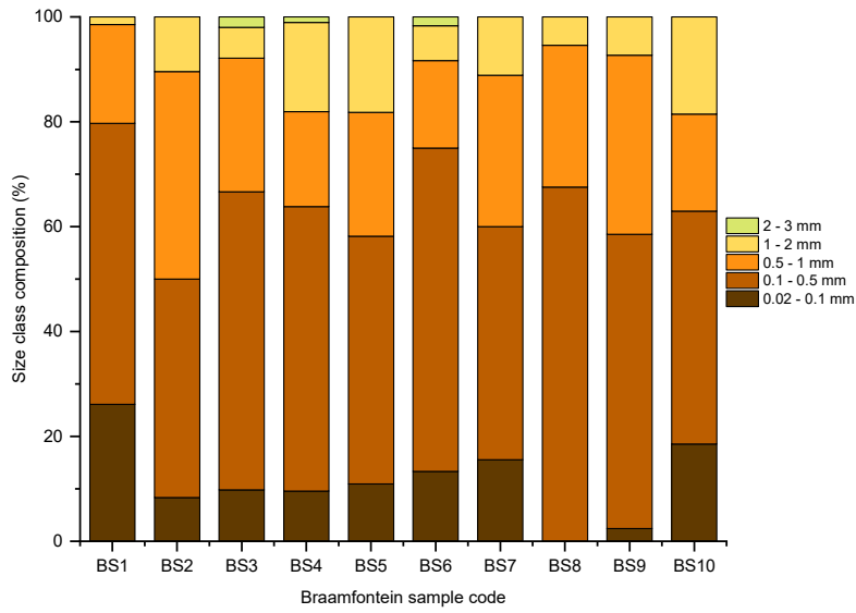
Figure S1. Distribution of microplastic a) shapes and b) sizes in Braamfontein samples
