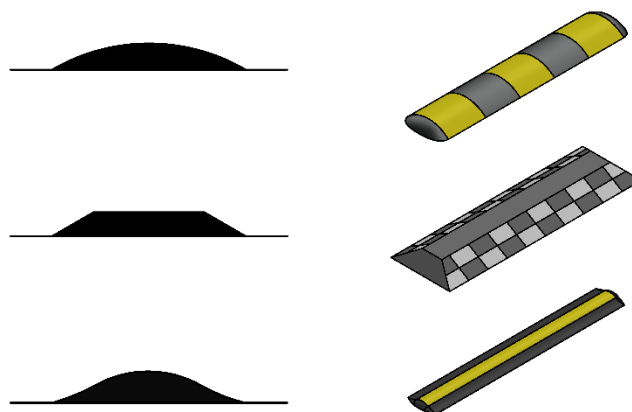
Figure 4. Global and lateral views:of speed bumps: circular (top); trapezoidal (middle); sinusoidal (bottom)
