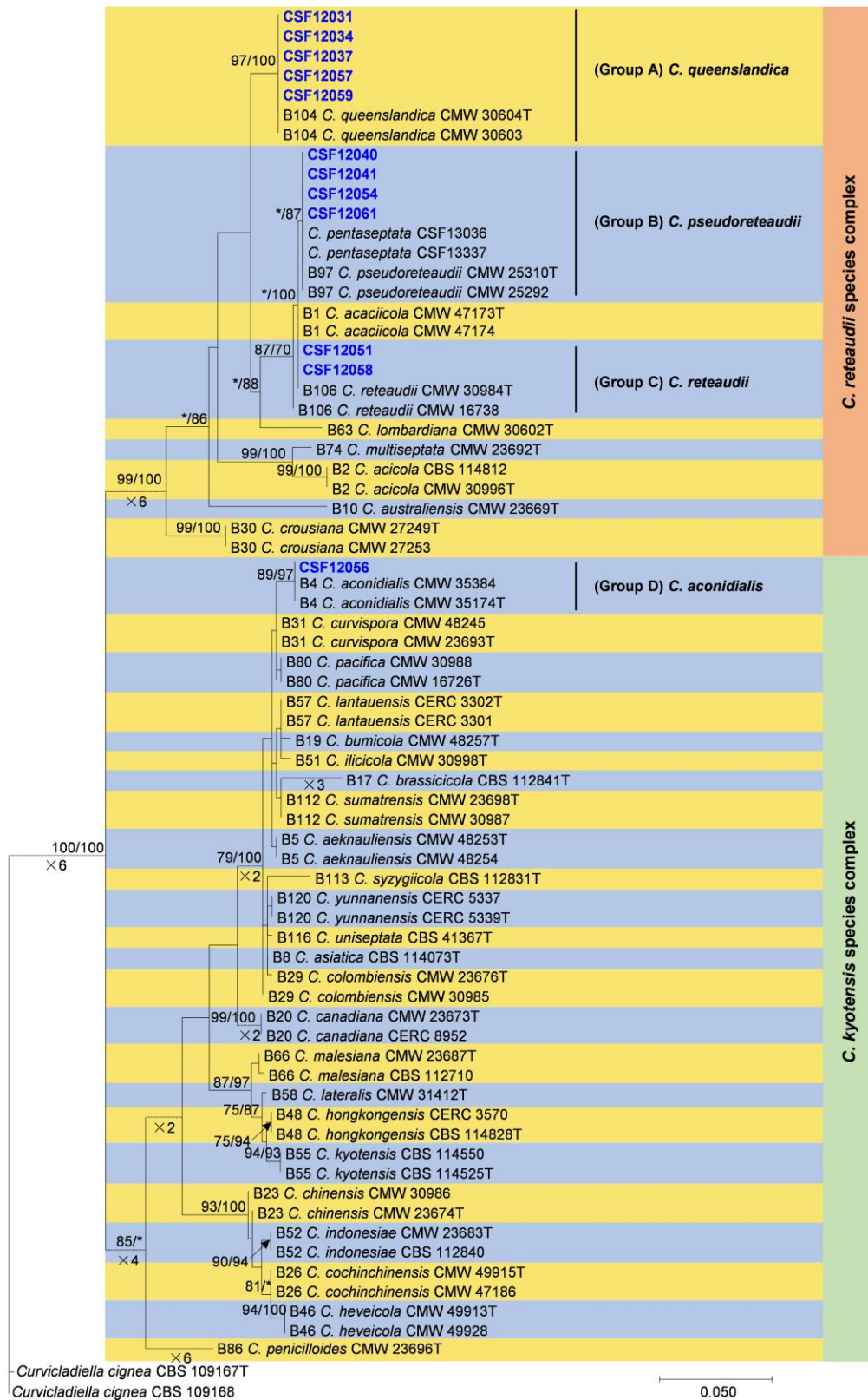
Supplementary Fig. S1. Phylogenetic trees obtained from Maximum Likelihood (ML) analyses of tef1 region for species in the C. reteauidii and C. kyotensis species complexes. Bootstrap support values \geq 70\% for ML and MP are indicated above the branches as ML/MP. Bootstrap support values < 70\% are marked with “*”. Isolates obtained in this study are highlighted in blue and in bold type; “T” represents ex-type isolates. “B” species codes are consistent with the published results in Liu et al. (2020). Curvuladiella cigna (CBS 109167 and CBS 109168) was used as the outgroup taxon.
