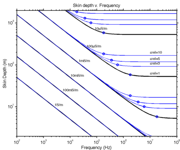
Fig. 6 Skin depth, frequency, and conductivity relation chart [14]
