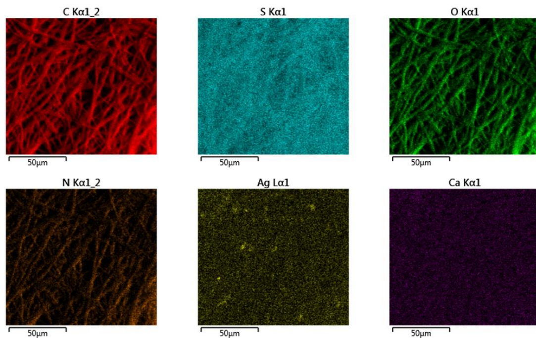
Figure S2 ESM/AgNPs EDS Map
