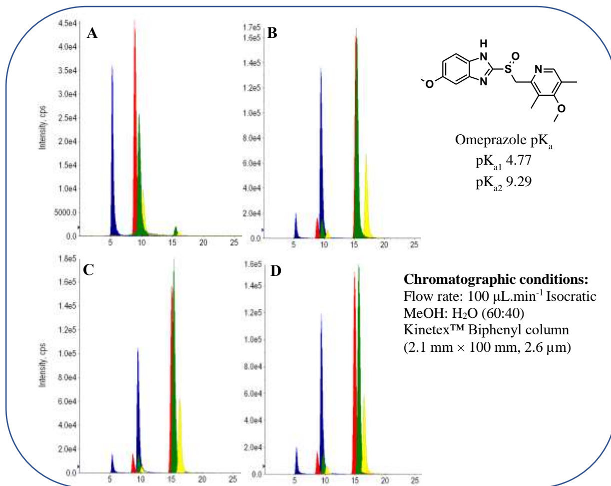
Supplementary Figure 1: Overlaid XIC of omeprazole (100 \text{ng}\cdot\text{mL}^{-1} ) in 50:50 methanol: water containing 0.1% formic acid (A), 10 mM ammonium formate (B), 10 mM ammonium acetate (C) and 5 mM ammonium bicarbonate (D) at different mobile phase conditions; pH 2.7 (blue peak), pH 3.9 (red peak), pH 6.5 (green peak) and pH 8.3 (yellow peak).
