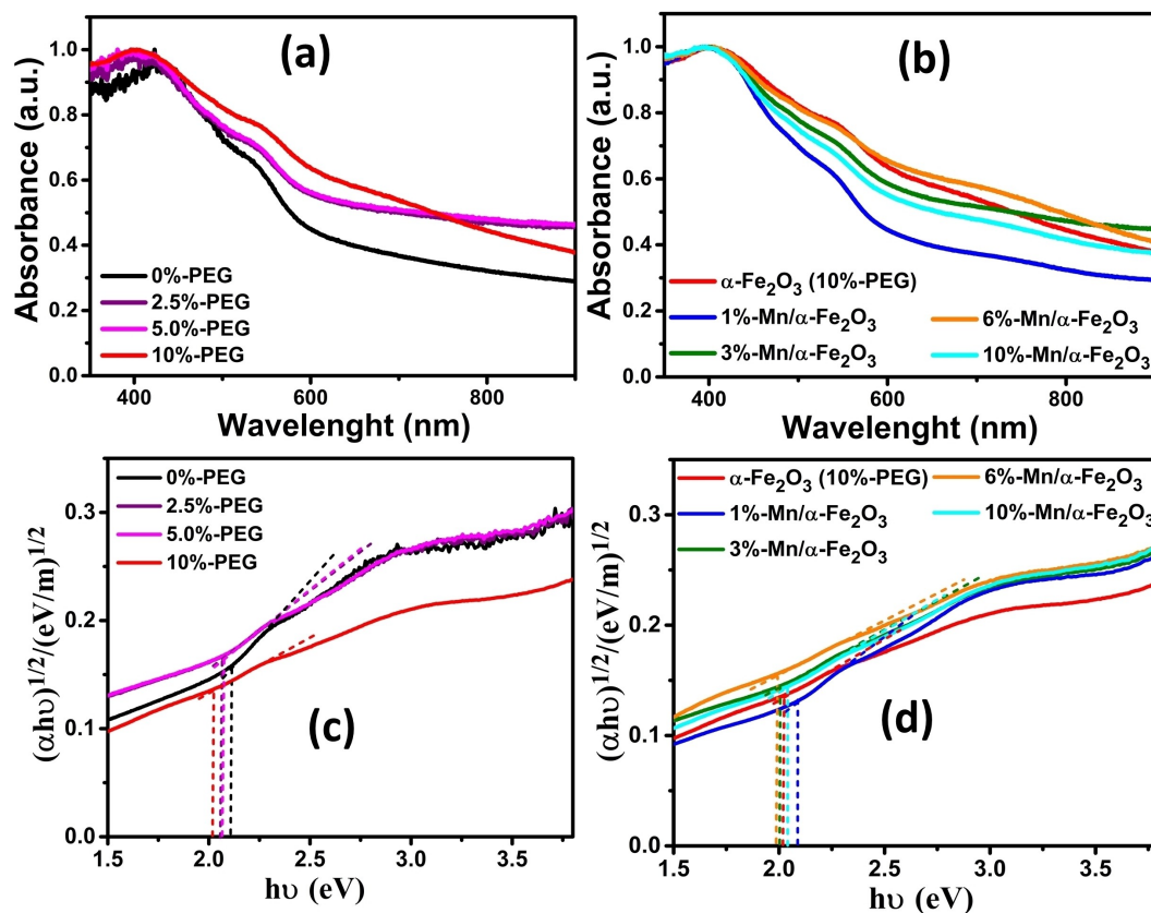
Figure 7. UV-Vis optical absorption of (a) pristine and (b) Mn-doped \alpha - \text{Fe}_2\text{O}_3 films: (c) and (d) present the Tauc plots for the approximation of the indirect bandgap of the pristine and doped samples, respectively.
