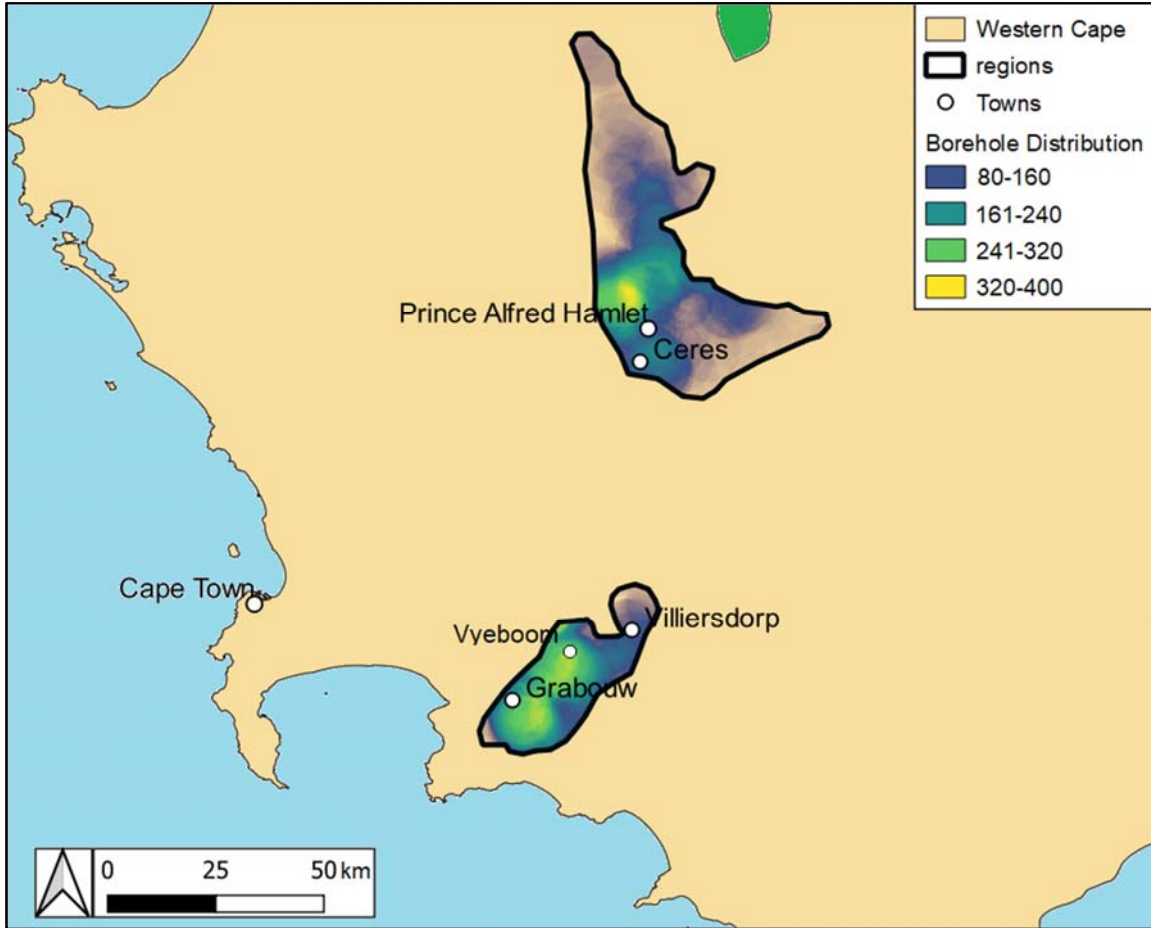
Fig S5: A map of the borehole distribution in the apple-growing regions. Adapted from the Department of Water and Sanitation (2021).
