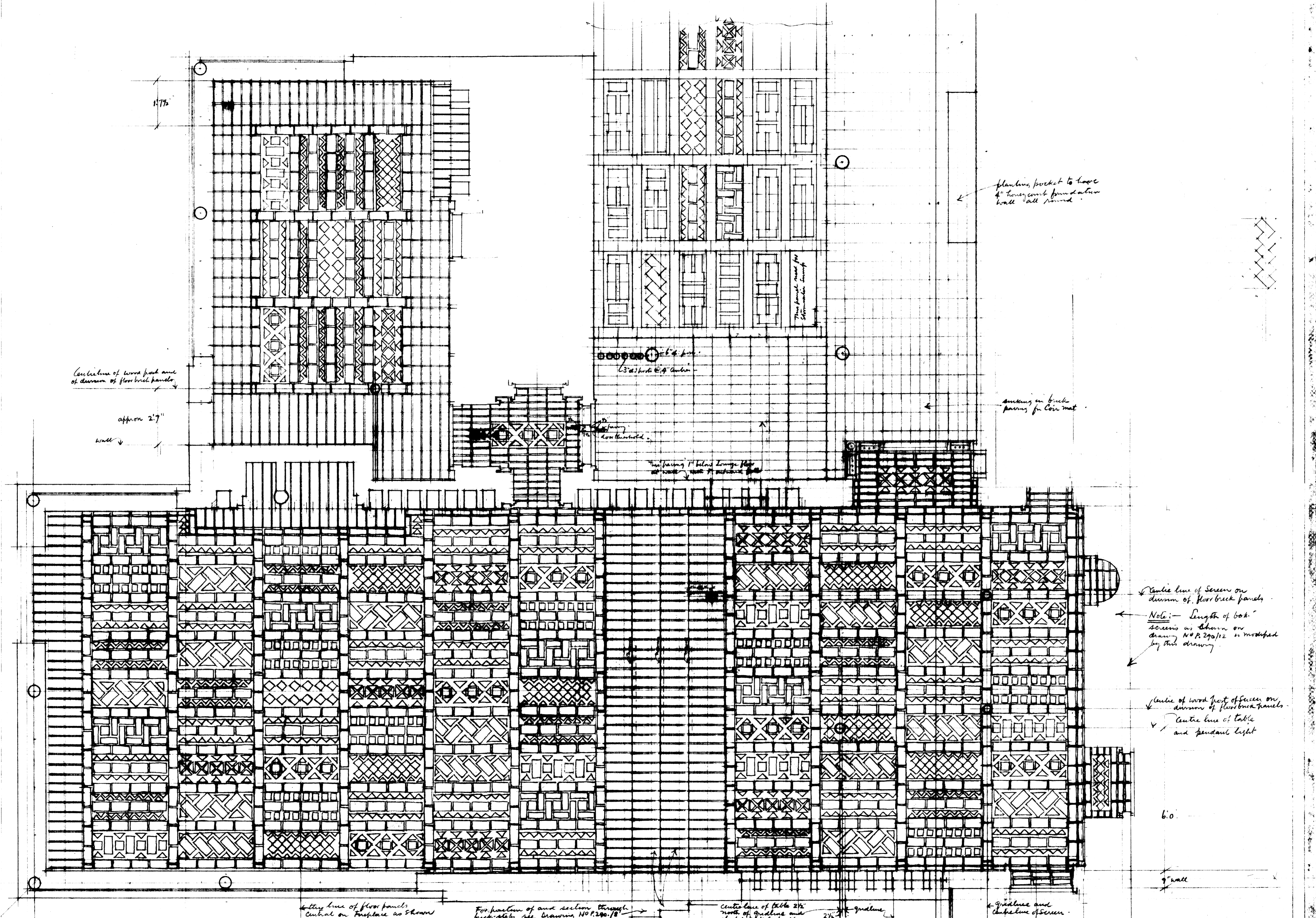
COURTYARD HOUSE ON ERF N° 80, ANTARES STREET, WATERKLOOF RIDGE, PRETORIA. for MR. H.M. MOKULIATY HALF INCH SCALE PLAN OF BRICK FLOOR "CARPETS" AND PAVINGS, ETC. NORMAN EATON & LOUW, ARCHITECTS, PRETORIA. NOVEMBER 1961
