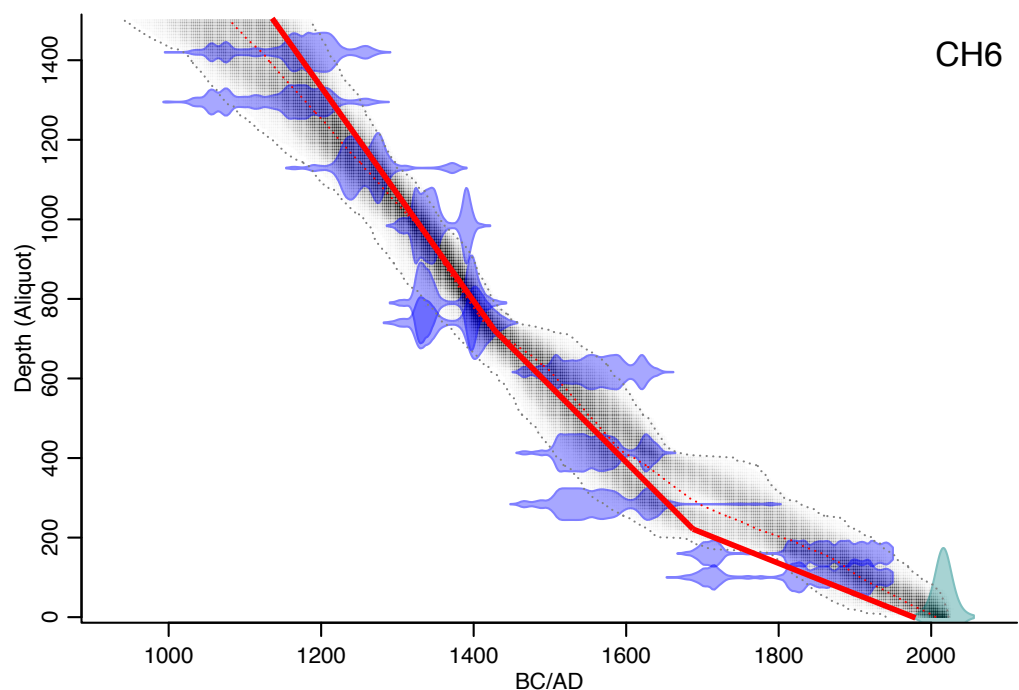
Figure S1. Age-depth model. The Bayesian accumulation (BACON) model is presented for samples CH3 and CH6. This model used the 19 radiocarbon dates (blue) calibrated using SHCal20 [78], which were presented in Table 1. Our linear age model for both samples can be seen in thick red lines, on top of the BACON model, for comparison.
