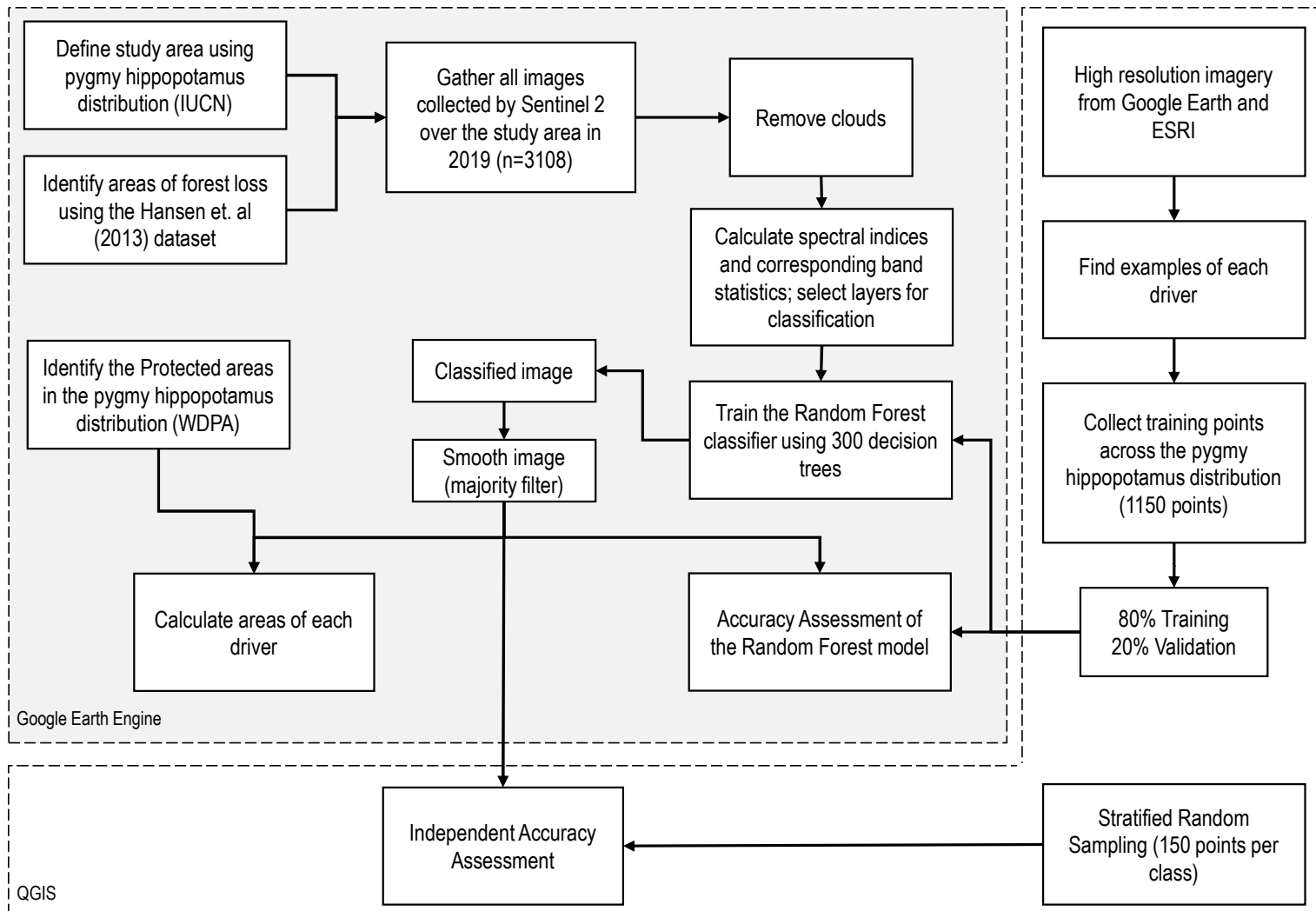
Figure S1: Image processing and classification workflow. Image acquisition and processing was done in Google Earth Engine, as well as model training and application of the model to the selected imagery. Training points and the independent accuracy assessment were done in QGIS.
