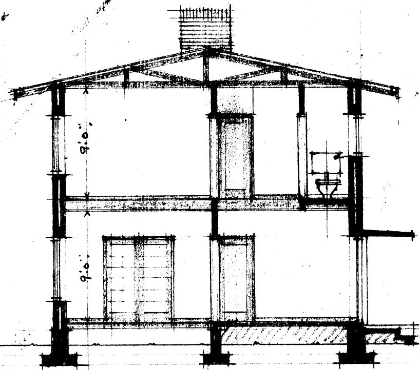
CROSS SECTION
