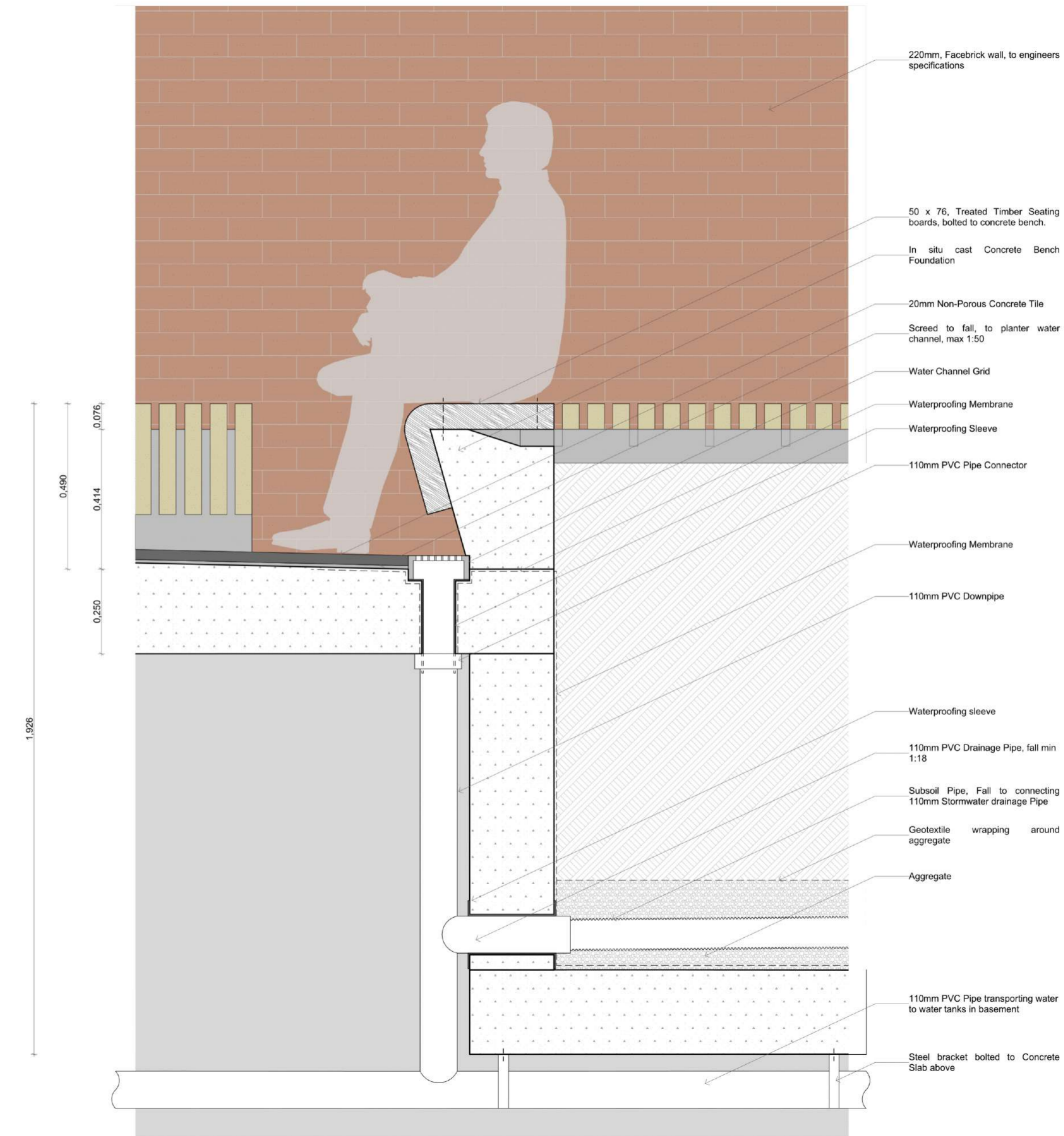
DETAIL 3 SCALE 1:10
