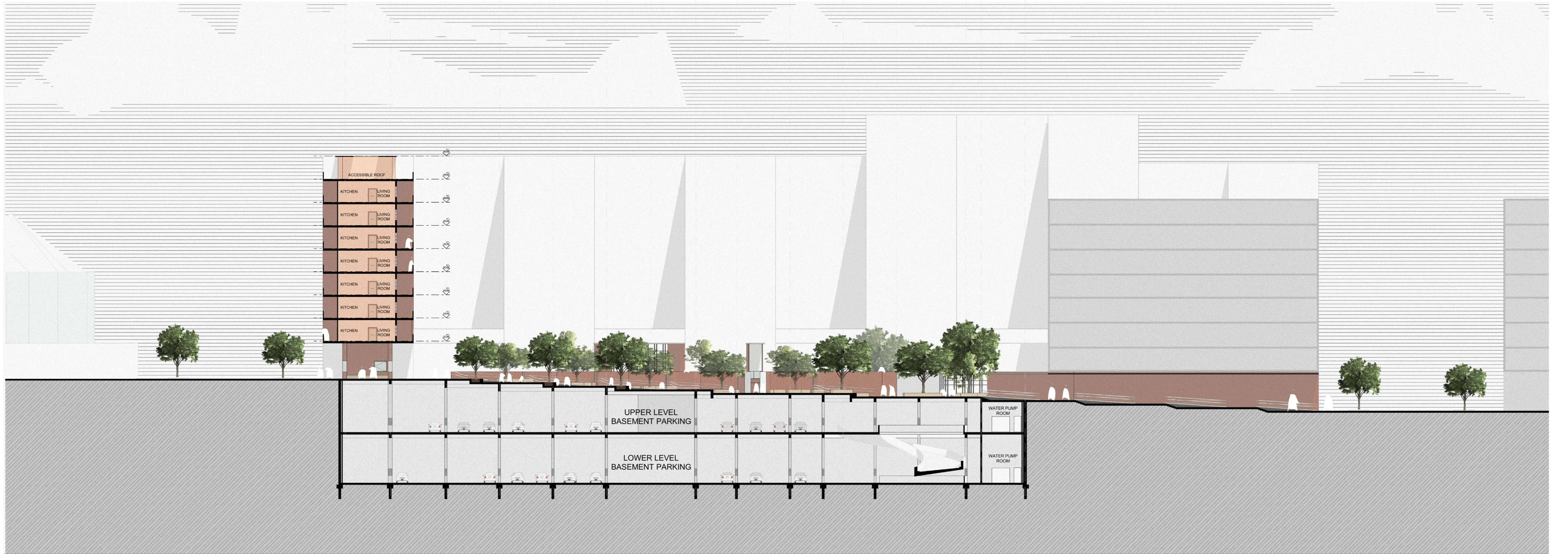
SECTION AA SCALE 1:200
