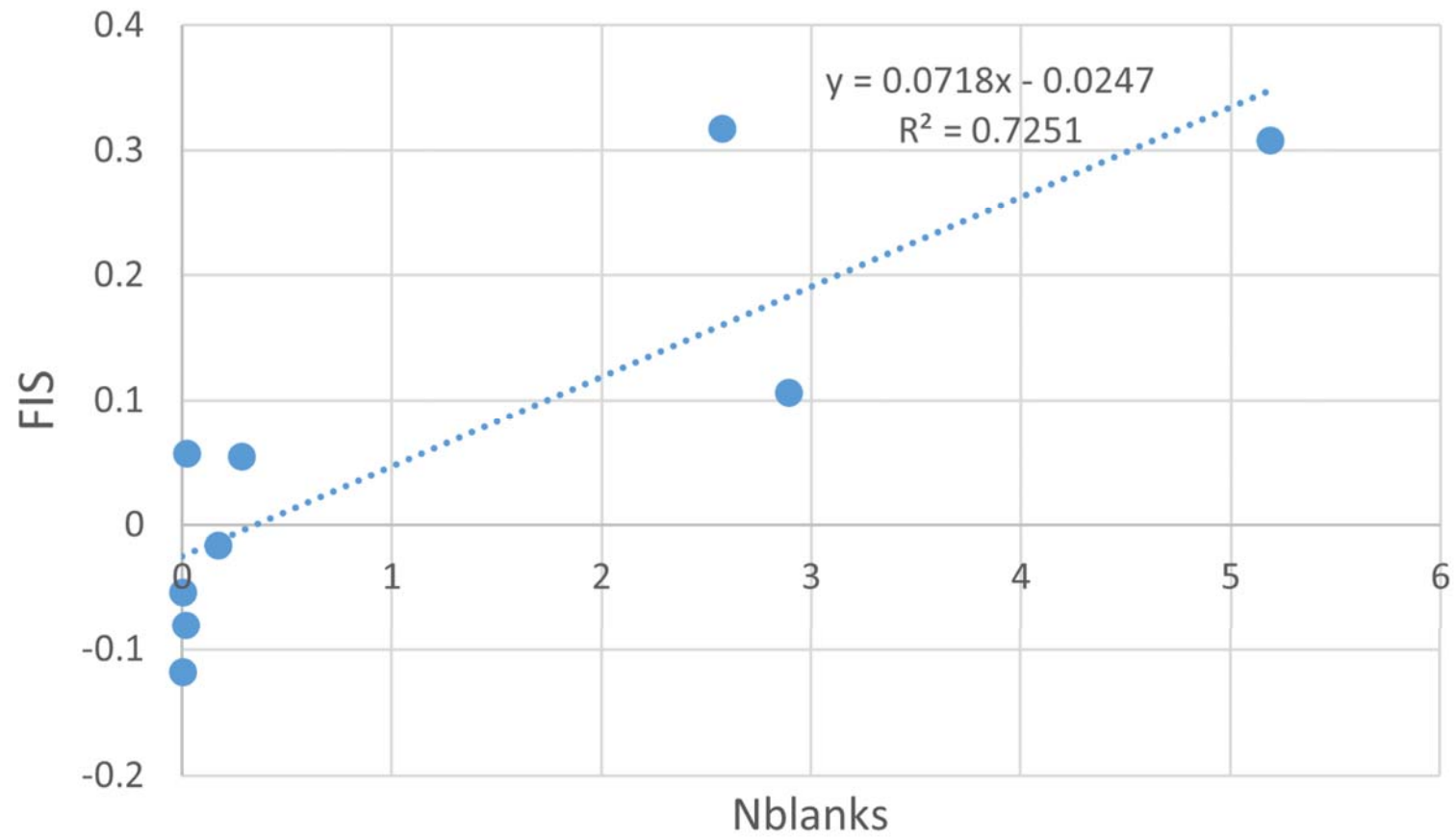
Supplementary Figure 7: Correlation between F_{IS} and FST (A) and between F_{IS} and number of blanks (B) for selected nine loci across field samples.
