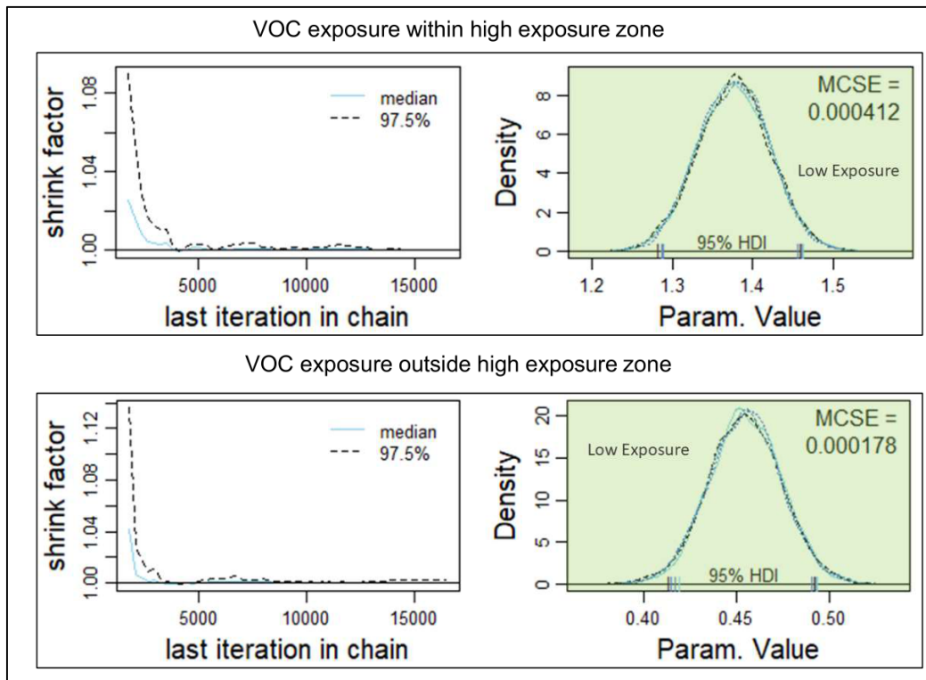
Figure S-3: VOC exposure within (top) and outside (bottom) high exposure zones – Convergence (left) and probability of exposure (right). Parameter values in \text{mg}/\text{m}^3
