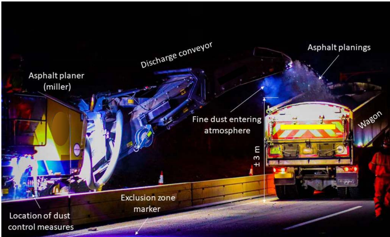
Figure S-1: Asphalt planer milling hardened asphalt and producing fine dust
