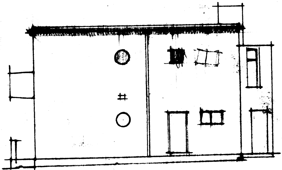
WEST ELEVATION
