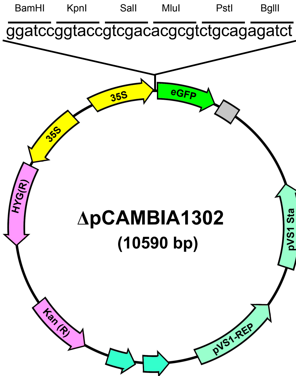
Supplementary Figure S5. Modified pCambia1302 vector.
