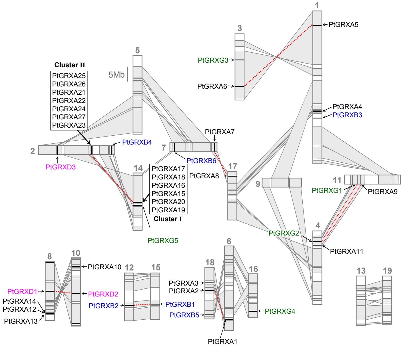
Supplementary Figure S1. Genomic localization of full-length Populus GRX genes. Regions that are assumed to correspond to homologous genome blocks are shaded gray and connected with lines. Paralogous GRX genes and clusters are indicated by red dashed lines within the gray-filled trapezoids.
