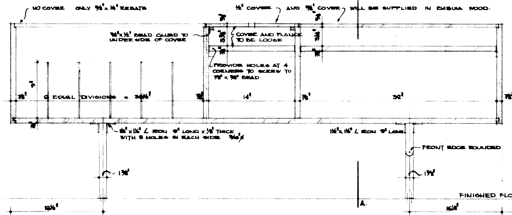
LONGITUDINAL SECTION THROUGH RECORD PLAYER
