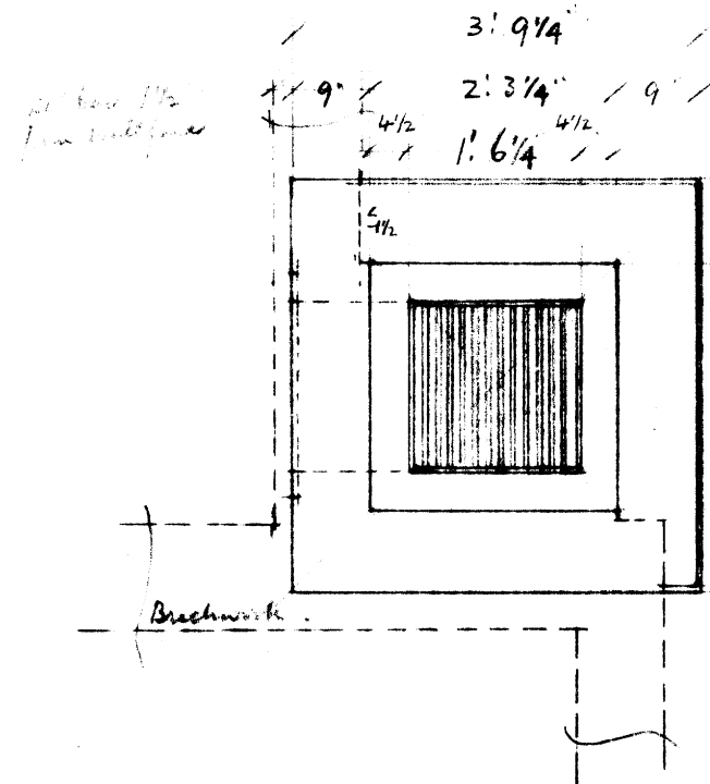
PLAN of METAL HEARTH
