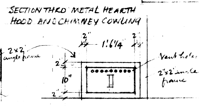
ELEVATION of ASH DRAWER & VENT
