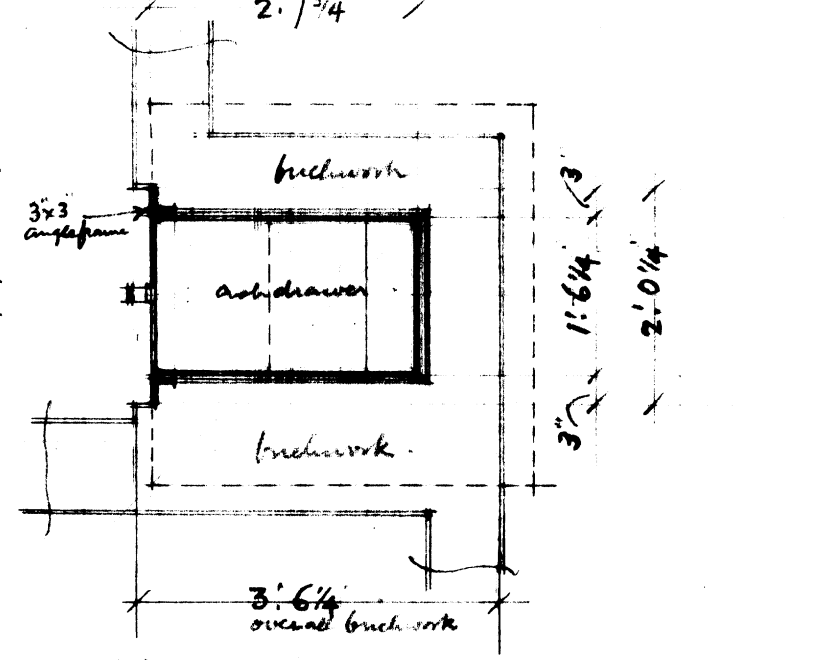
PLAN of ASH DRAWER BELOW HEARTH
