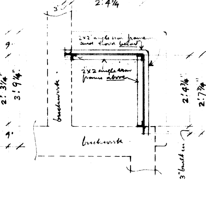
PLAN of METAL HOOD
