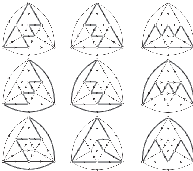
FIGURE A1 All (n - 1) -cycles for the 9-vertex graph from Figure 2 that are needed to apply Lemma 3. Note that when missing the top or bottom vertex of the \theta -subdigraph the cycle indeed uses one of the remaining edges, but not the central edge
