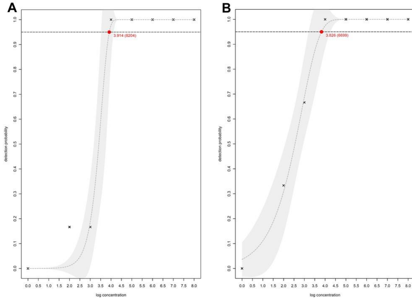
Figure S2. Non-linear modeling of the probability of detection for the AY-SA-specific LAMP (A) and real-time AY-SA-specific PCR assays (B). For both assays two parameter Weibull function fitted the best to experimental data. Log concentration, expressed as \log(\text{target dsDNA molecules/ml}) ; dotted line, 95% probability of detection.
