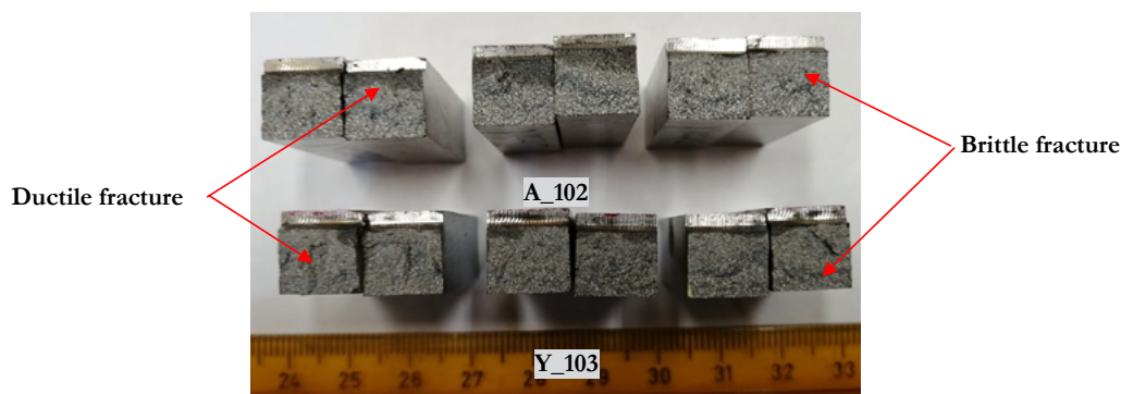
Figure 12: Macro photograph images of representative broken Charpy U-notch (2 mm) specimens for the rail samples showing a mixture of ductile and brittle failure mode
