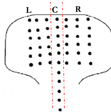
Figure 3: Rockwell C hardness traverse indentation map
