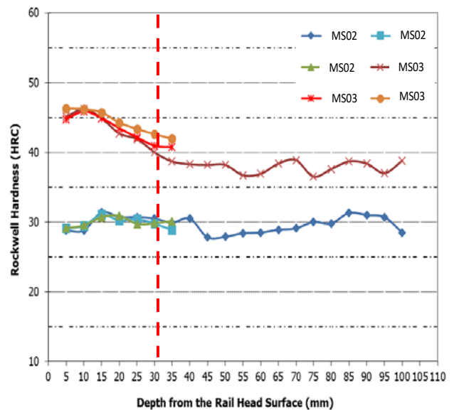
Figure 10: Graphical presentation of the hardness values of the railway cross-sections
