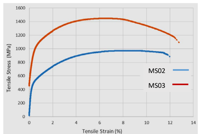
Figure 11: Tensile stress vs tensile strain
