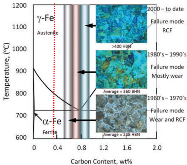
Figure 1: Evolution of rail steel metallurgies, hardness levels, and failure modes in the past 50 years 11
