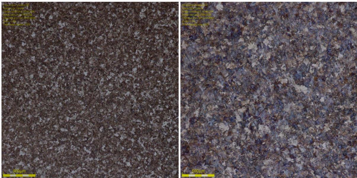
Figure 6: Microstructures of MS03 at 100X (low) magnification (a) near the rail head surface (Position A) and (b) at the centre (Position B)
