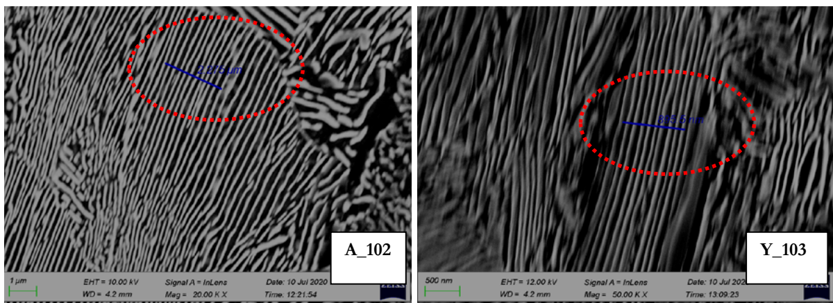
Figure 9: Scanning electron microscopy (SEM) images of MS2 and MS3 rail showing the measurement of the inter-lamellar spacing using the line intercept method
