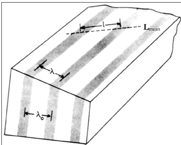
Figure 8: Schematic illustrations of various spacing in an ideal lamellar structure 14-16
