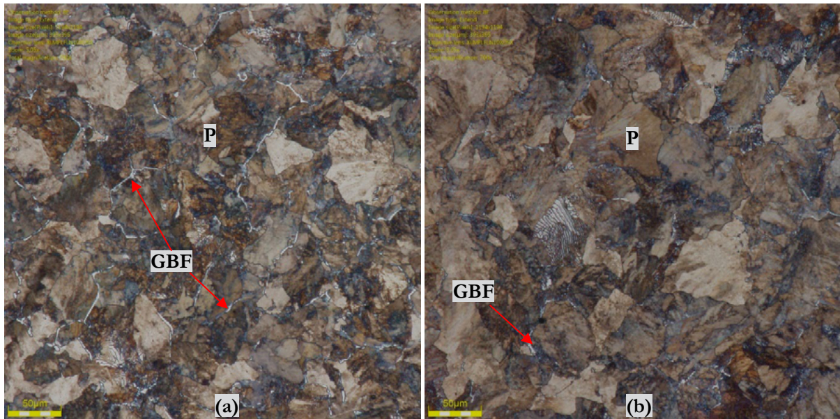
Figure 5: Microstructures of MS02 at high magnification (a) near the rail head surface (Position A) and (b) at the centre (Position B) showing pearlite (P) and grain boundary pearlite (GBF)
