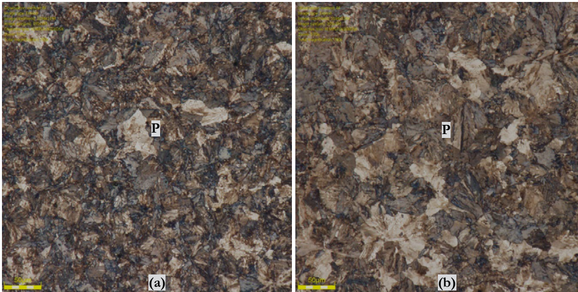
Figure 7: Microstructures of MS3 at high magnification (a) near the rail head surface (Position A) and (b) at the centre (Position B) showing pearlite (P)
