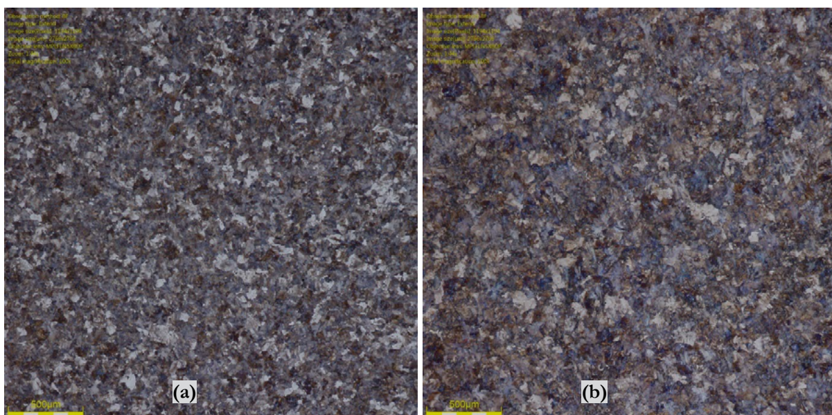
Figure 4: Microstructures of MS02 at 100X (low) magnification (a) near the rail head surface (Position A) and (b) at the centre (Position B)
