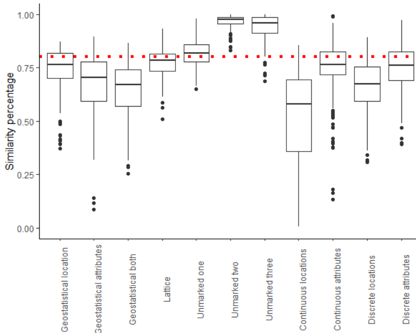
Figure 3. Results from applying the proposed spatial similarity test to the simulated spatial data being 80% identical. The red line indicated 0.8.
