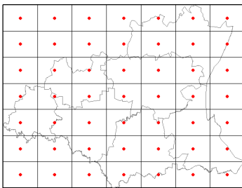
Figure 1. Illustration of how the spatial domain for lattice data is divided into pixels with m = 7 . The red dots represent the u_j 's.
