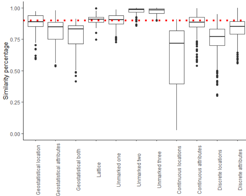
Figure 4. Results from applying the proposed spatial similarity test to the simulated spatial data being 90% identical. The red line indicated 0.9.
