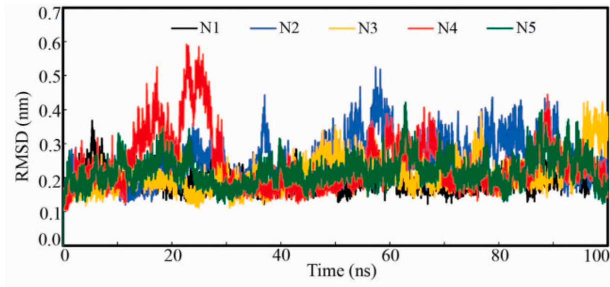
Fig. 5. RMSD of Nsp15 endoribonuclease backbone bound with N1, N2, N3, N4 and N5. All Nsp15 backbone except bound with N4 found to be equilibrated from the beginning of the simulation. Nasp15 backbone bound with N4 was seen equilibrated after about 30ns.
