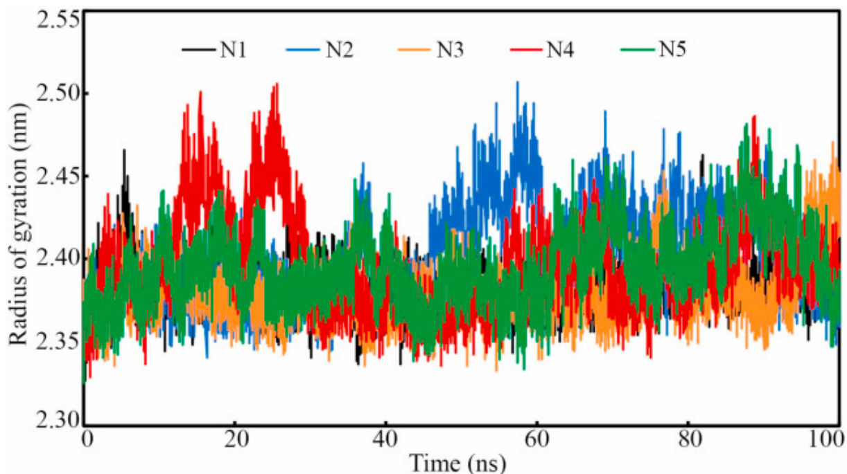
Fig. 7. Radius of gyration for Nsp15 endoribonuclease. The range of the radius of gyration was found 2.30–2.50 nm. All trajectories showed the compactness of each complex throughout the simulation.
