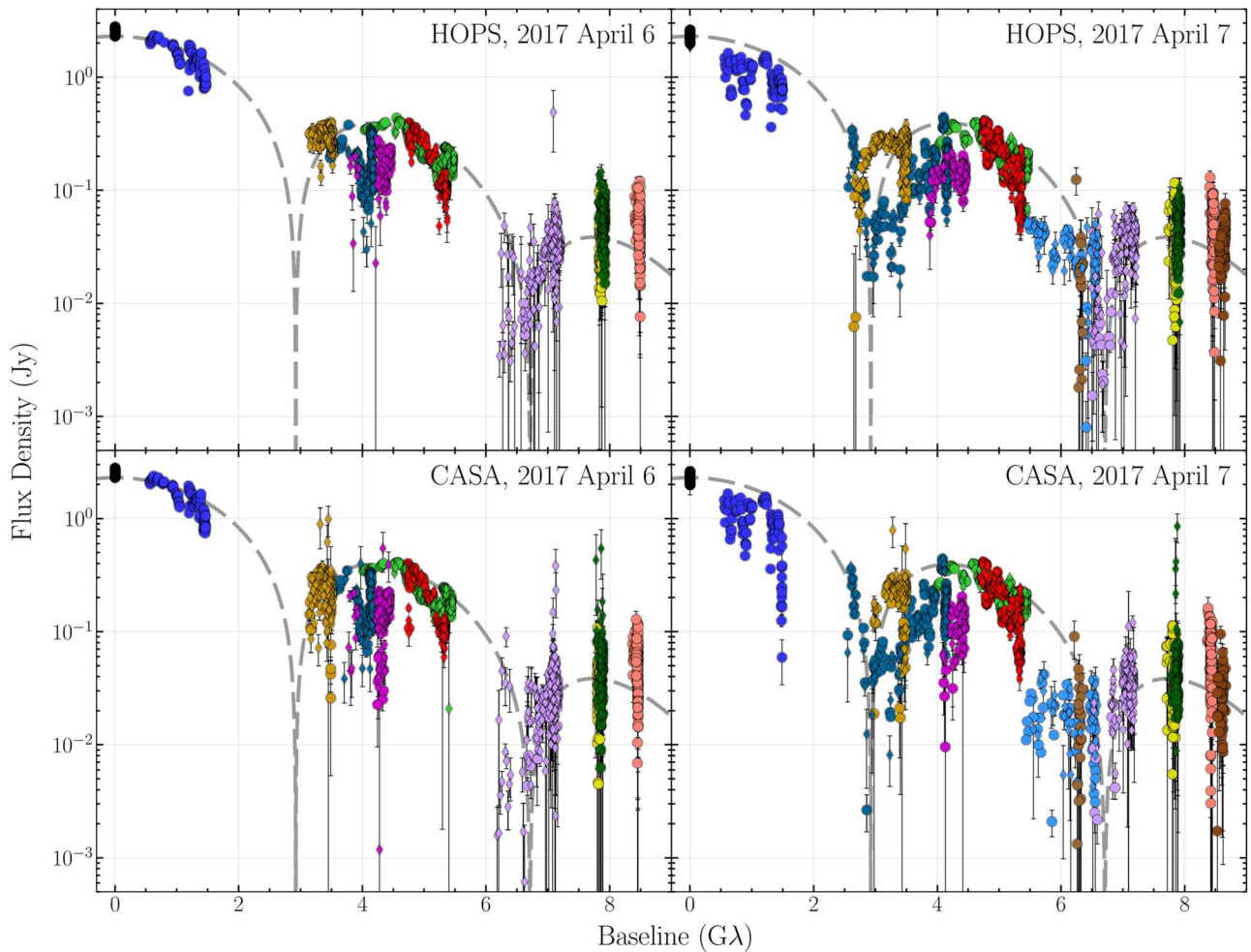
Figure 9. Measured correlated flux densities of Sgr A* on April 6 and 7 of the HOPS (top) and CASA (bottom) data overplotted with a thin (unresolved) ring model with a \sim 50 \mu\text{s} diameter, which has been blurred with a 23 \mu\text{s} FWHM circular Gaussian source (Papers III and IV). Flux densities have been calibrated based on estimated station SEFDs, measured light curves (Section 3.2.1), and calibrator gain transfers (Section 3.2.2). The data are averaged in 120 s bins, which causes phase coherence losses in a few scans. Error bars denote \pm 1\sigma uncertainty from thermal noise. Detections are color-coded by baselines, as in Figure 8. Redundant baselines are shown with different symbols: circles for baselines to ALMA and SMA; diamonds for baselines to APEX and JCMT.
