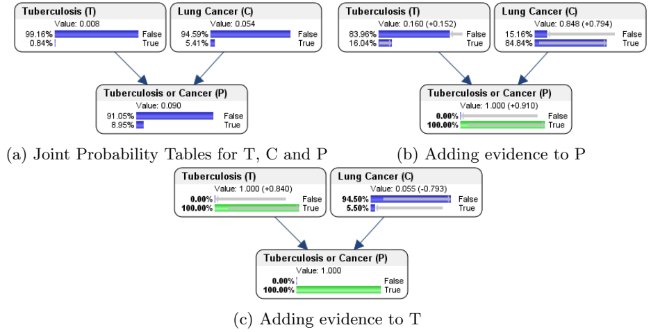
Figure 2: Belief Updating for T, C and P
