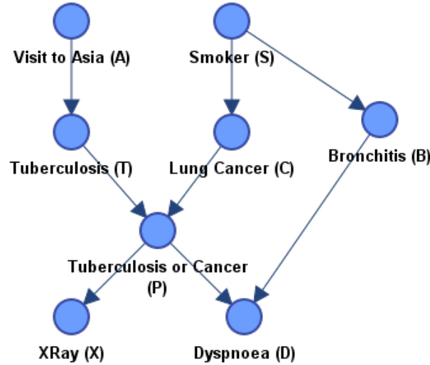
Figure 1: Asia Bayesian network
