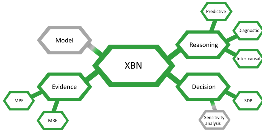
Figure 7: A schematic view of XBN
