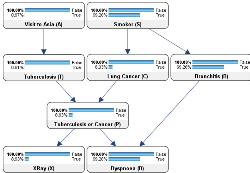
Figure 3: Initial MPE for Asia Bayesian network
