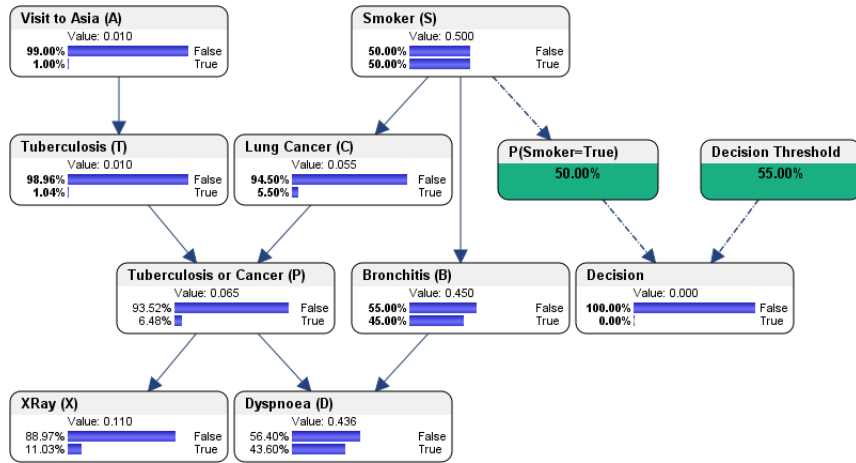
Figure 5: Addition of decision node in Asia network
