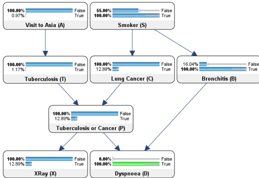
Figure 4: Updated MPE for Asia Bayesian network
