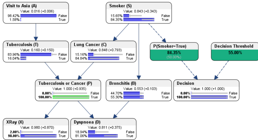
Figure 6: Updated decision for Asia network
