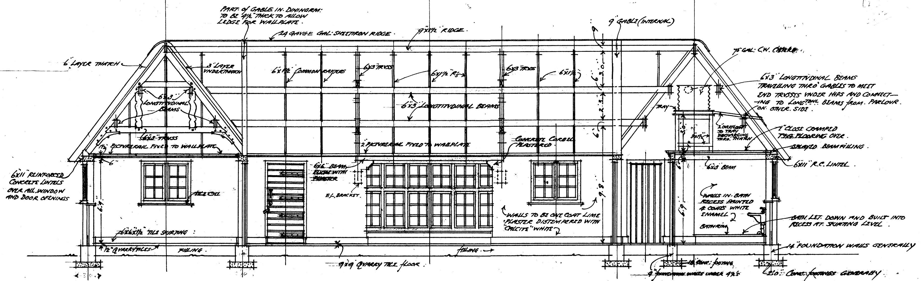
LONGITUDINAL SECTION "BC" ON CENTRELINE.
