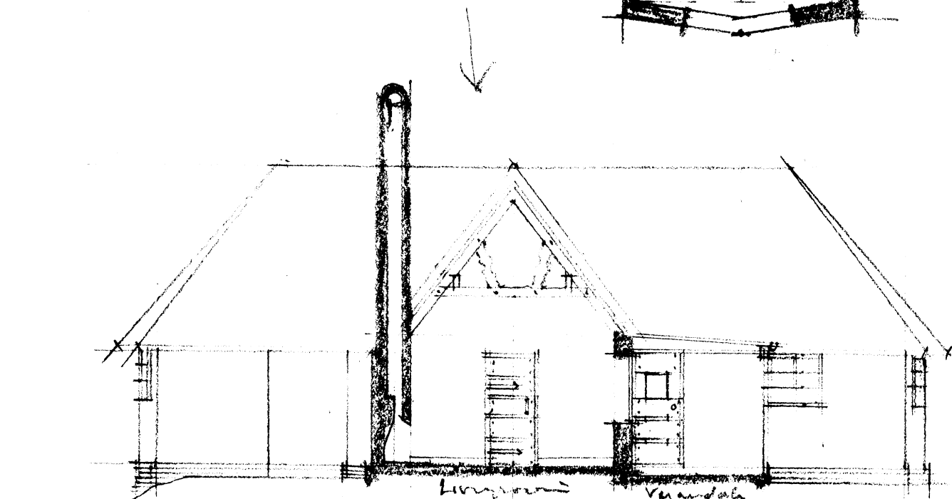
SECTION THRO' LIVING ROOM Looking West
