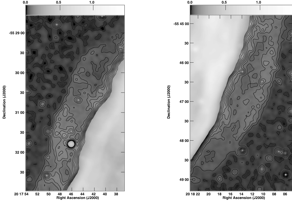
Figure 7. Portions of the cocoons surrounding the northern (left-hand panel) and the southern relic jets (right-hand panel) are shown with contours at T_b = 0.25 \text{ K} \times 1, 2, 3, \dots, 10 to emphasize their sharp inner and outer boundaries. The average brightness temperature in the cocoons is \langle T_b \rangle \sim 0.5 \text{ K} . The logarithmic grey scale spans -0.12 \text{ K} = -0.008 \text{ mJy beam}^{-1} (black) to +20 \text{ K} = +1.46 \text{ mJy beam}^{-1} (white) as indicated by the scale bar at the top.
