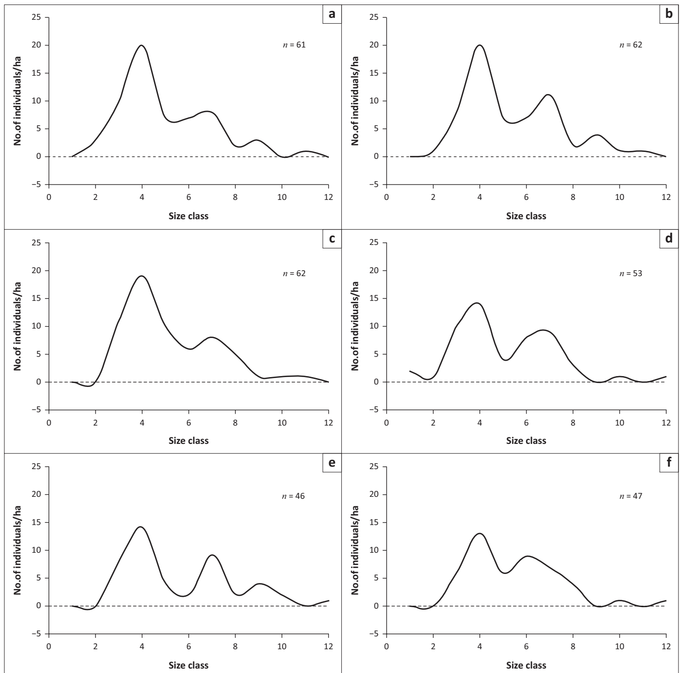
FIGURE 5: Size class distribution curves of Vachellia erioloba individuals at the Grootkolk site in the various survey years. (a) 1986; (b) 1984; (c) 1986; (d) 1989; (e) 1994; (f) 1996; (g) 1999; (g) 2008; (i) 2016.
