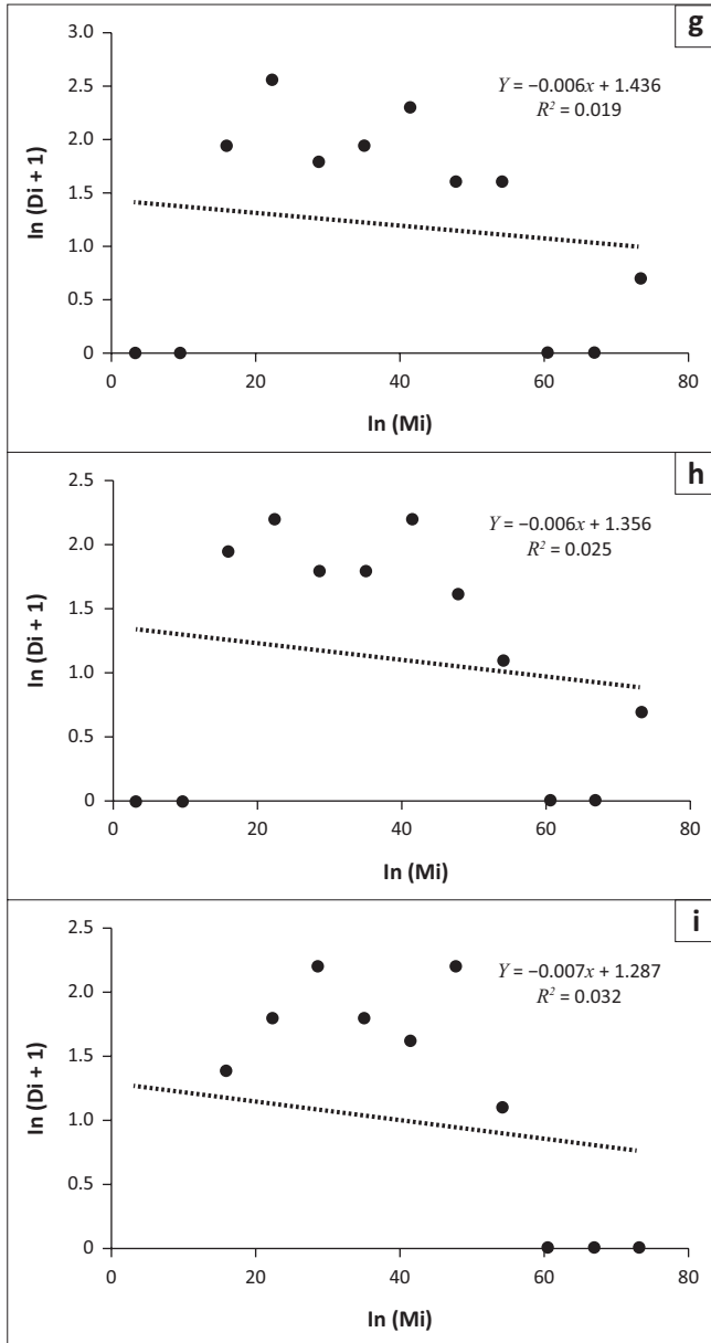
FIGURE 1-A1 (Continues...): Linear regressions fitted on the \ln(M_i) against \ln(D_i + 1) of live trees at Grootkolk in the Kalahari Gemsbok National Park in (a) 1979, (b) 1984, (c) 1986, (d) 1989, (e) 1994, (f) 1996, (g) 1999, (h) 2008 and (i) 2016, where M_i , midpoint of the size class and D_i , density of individuals.
