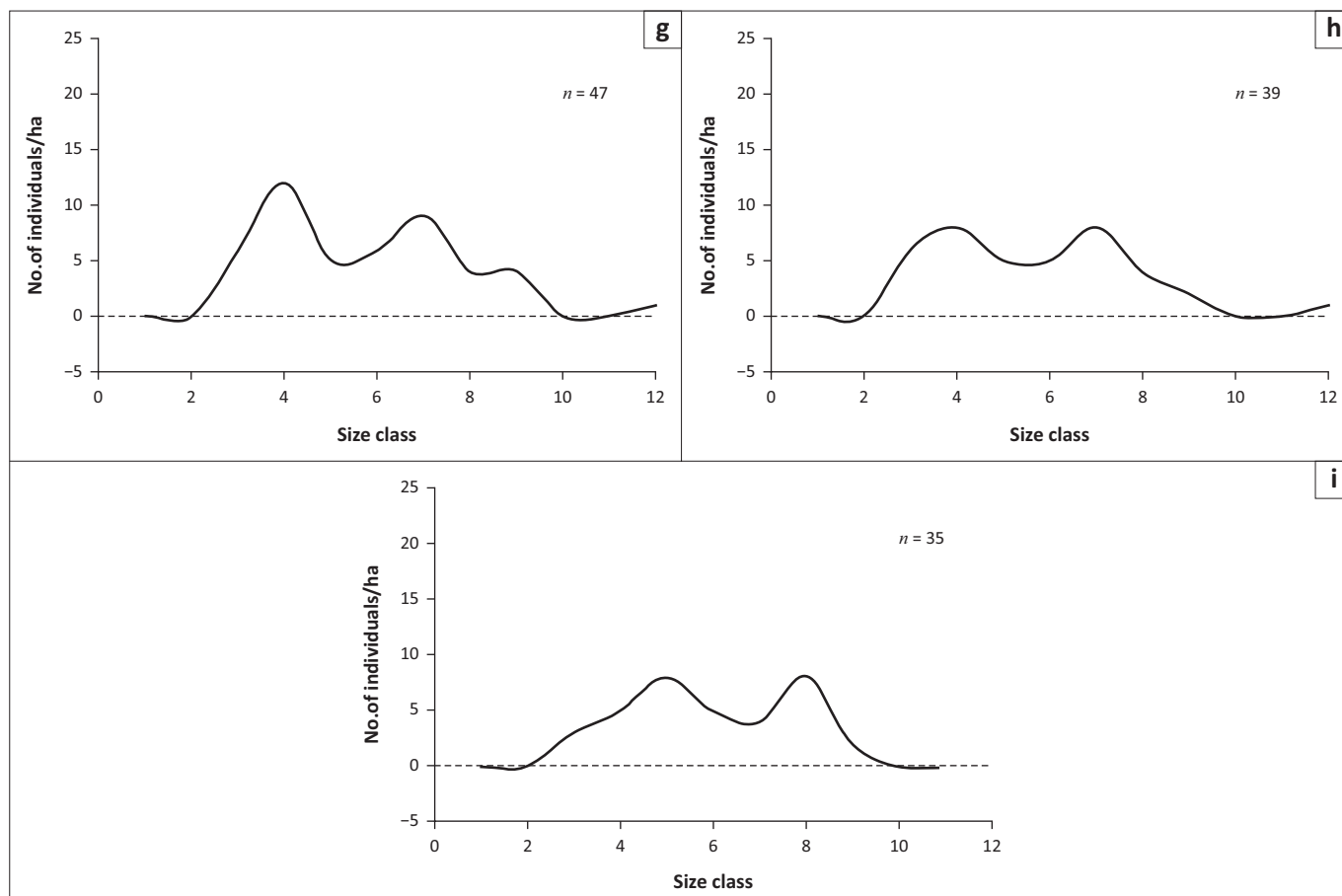
FIGURE 5 (Continues...): Size class distribution curves of Vachellia erioloba individuals at the Grootkolk site in the various survey years. (a) 1986; (b) 1984; (c) 1986; (d) 1989; (e) 1994; (f) 1996; (g) 1999; (g) 2008; (i) 2016.
