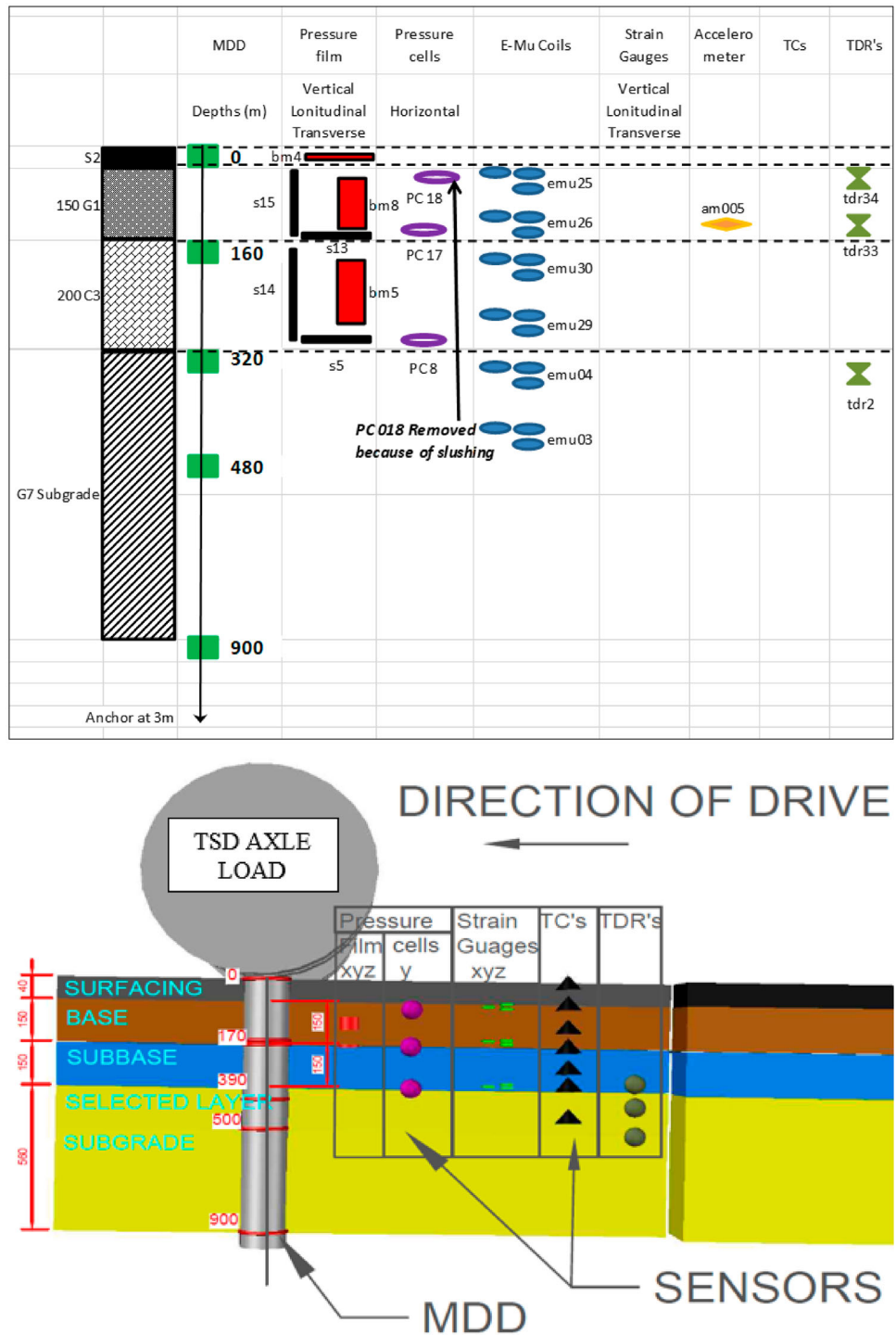
Figure 2. Instrumentation of the pavement systems.
