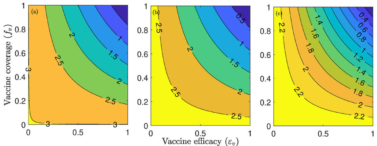
Fig. 8. Contour plots of the control reproduction number ( \mathcal{R}_c ), as a function of vaccine coverage ( f_v ) and vaccine efficacy ( \epsilon_v ) for (a) 10% mask compliance, (b) 30% mask compliance, and (c) 50% mask compliance. Parameter values used are as given in Table 3 with various values of c_M .
