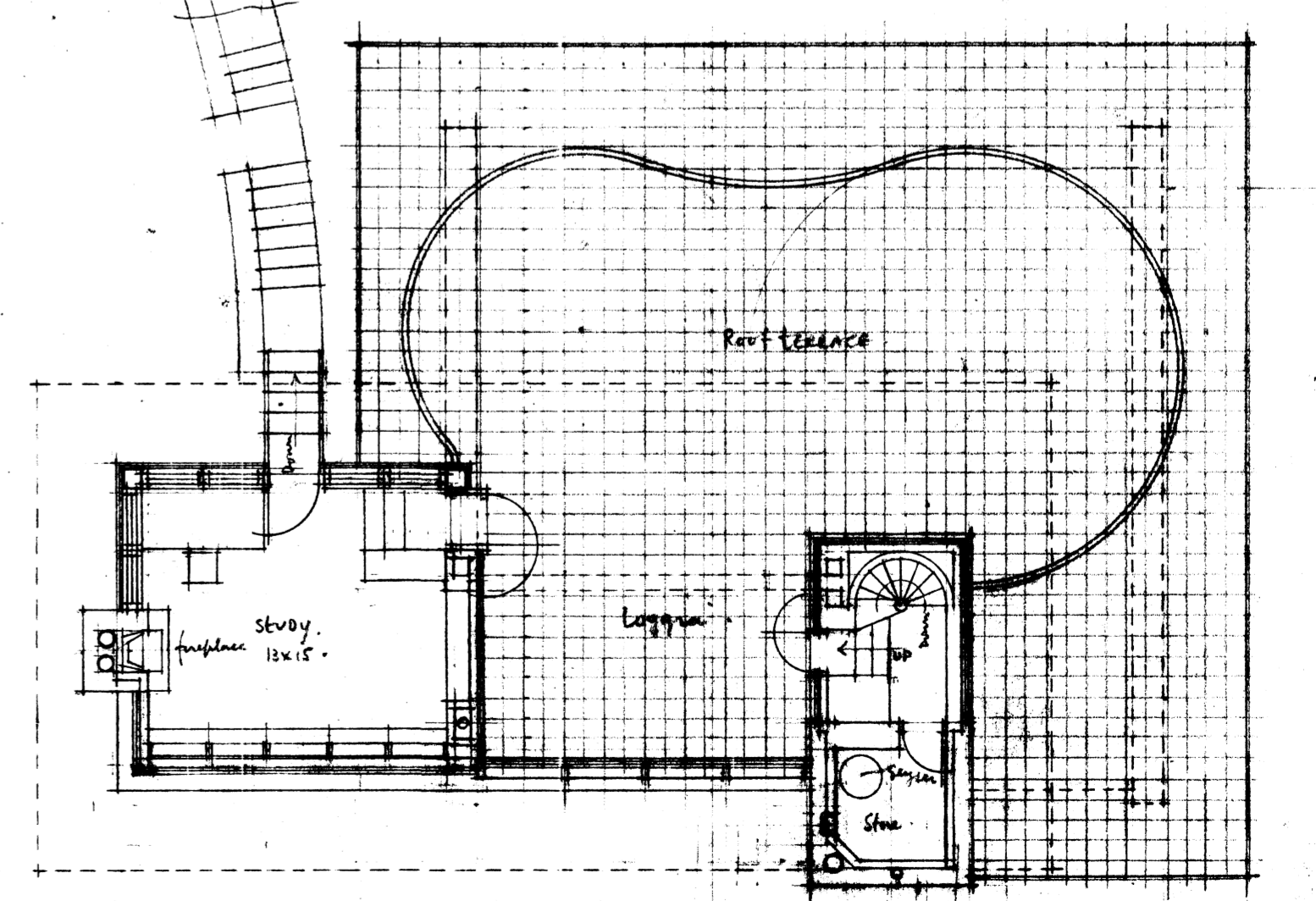
PLAN of ROOF TERRACE LEVEL.
