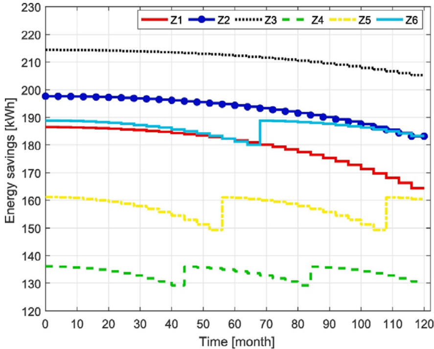
Fig. 4. Energy savings in each zone under Scenario 3.
