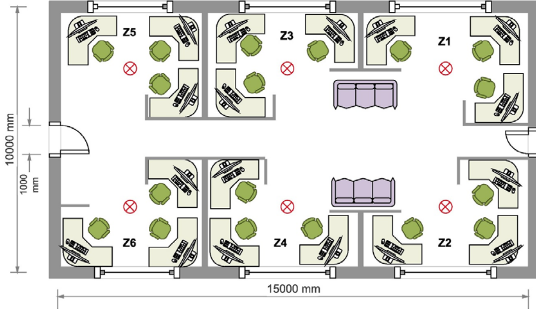
Fig. 1. Layout of the office under study.
