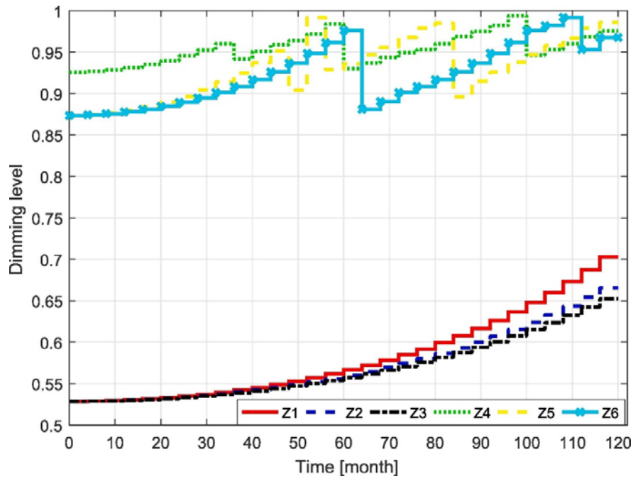
Fig. 6. Dimming level in each zone under Scenario 4.
