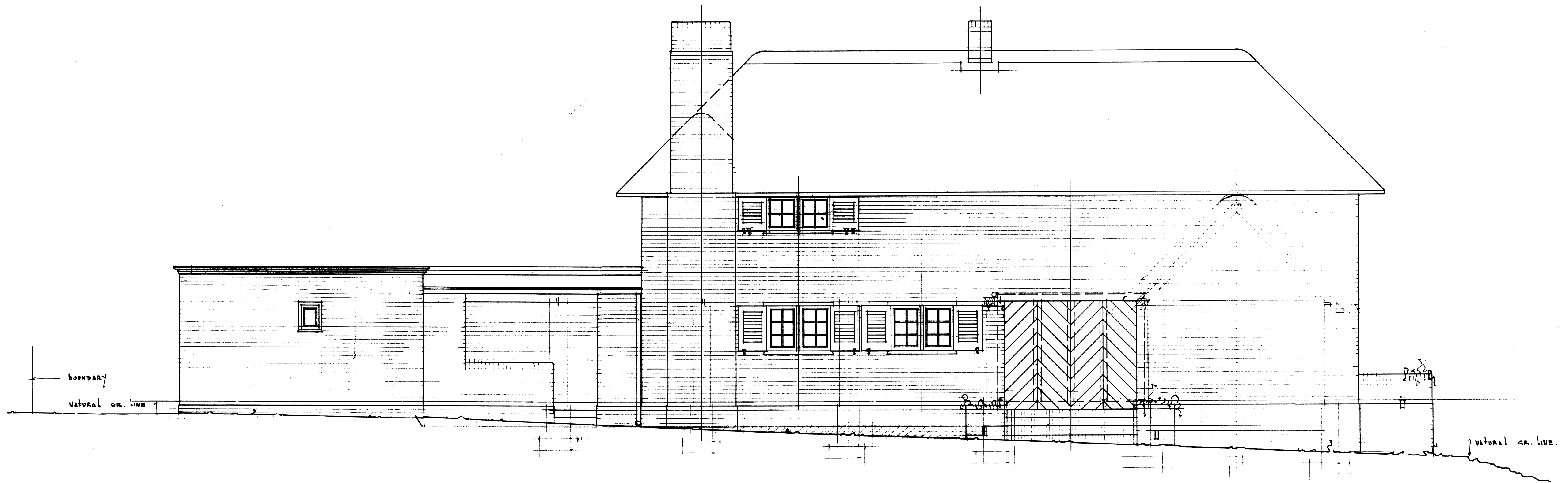
WEST ELEVATION
