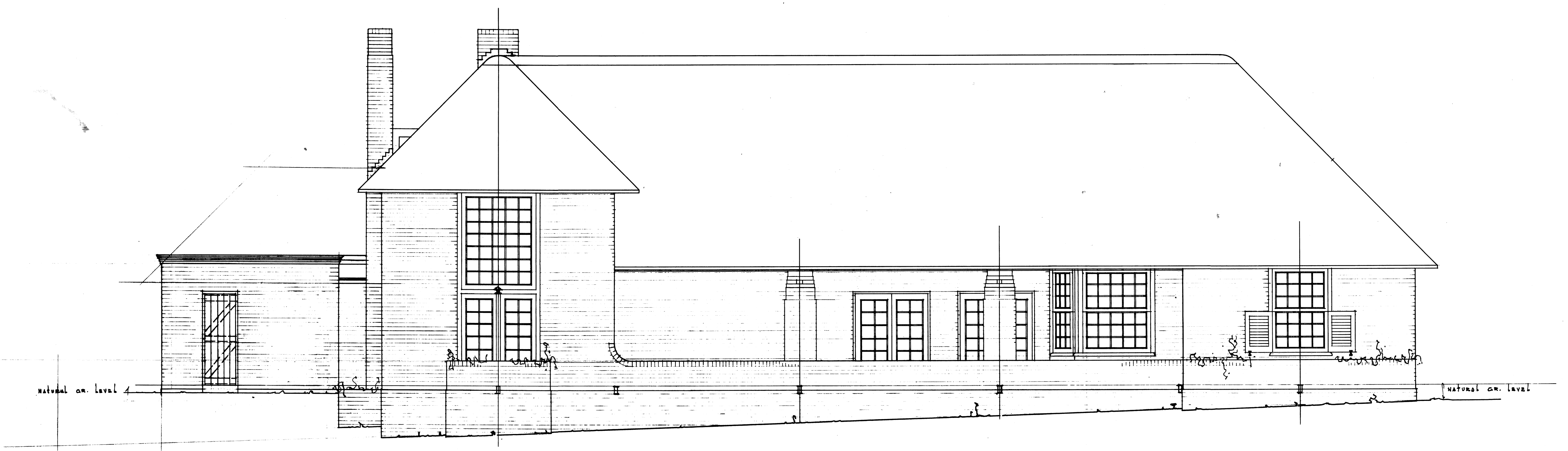
SOUTH ELEVATION
